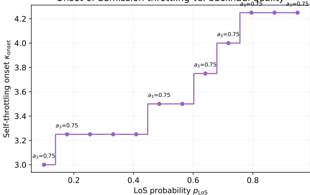
Onset of admission throttling vs. backhaul quality
