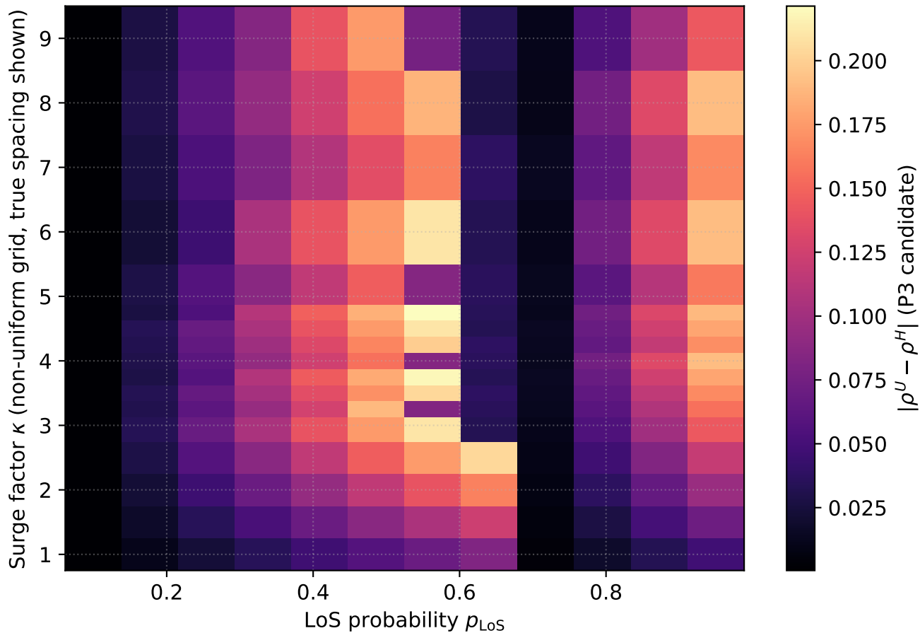
P3 stage-utilization balance across surge and backhaul quality
