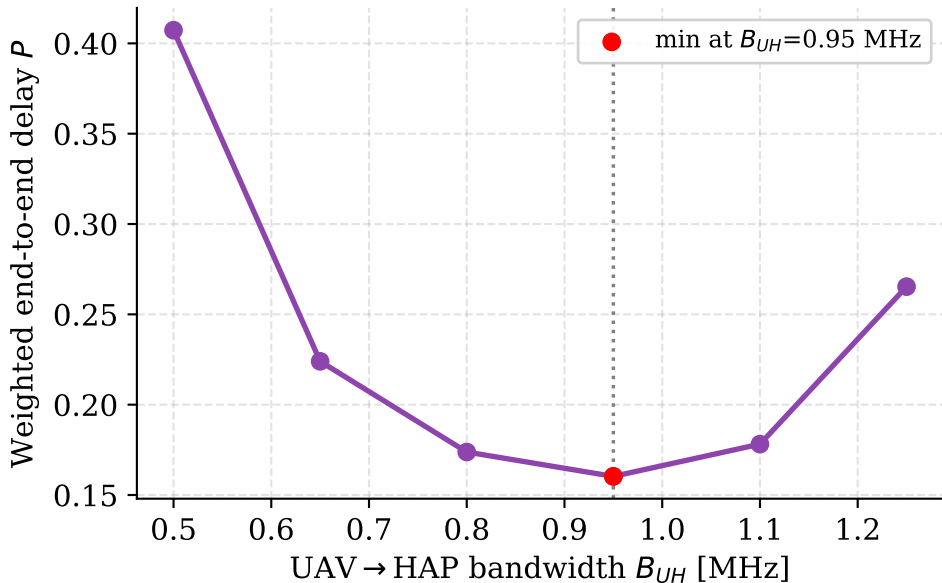
Weighted delay vs. bandwidth split ( B_{tot} = 2 MHz)
