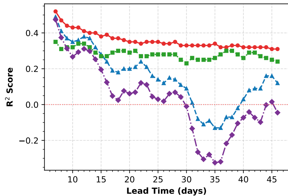
(a) R^2 across different lead times.
