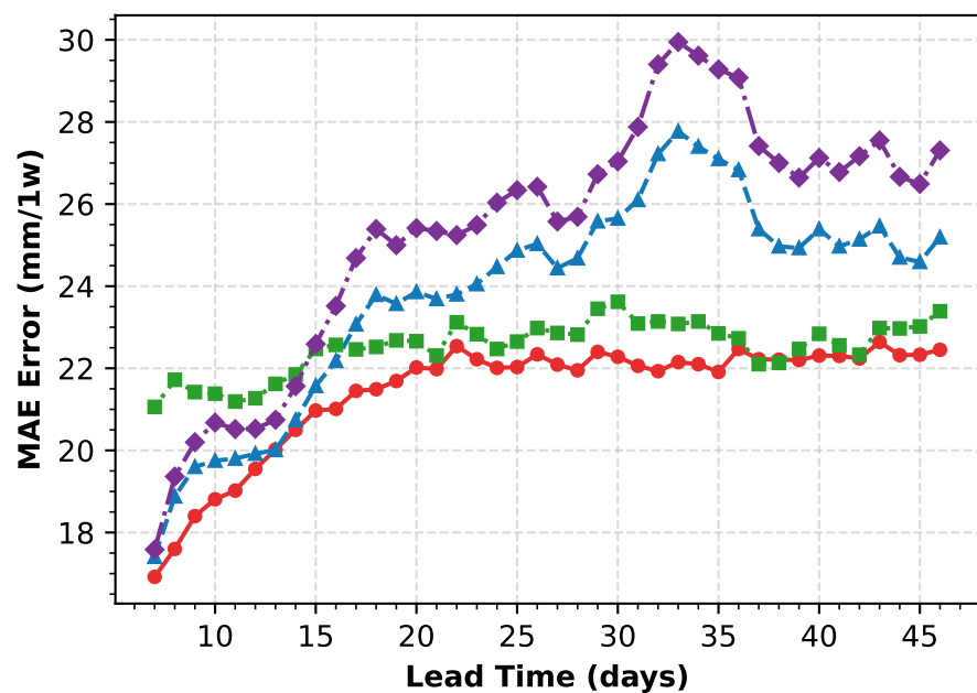
(c) MAE across different lead times.
