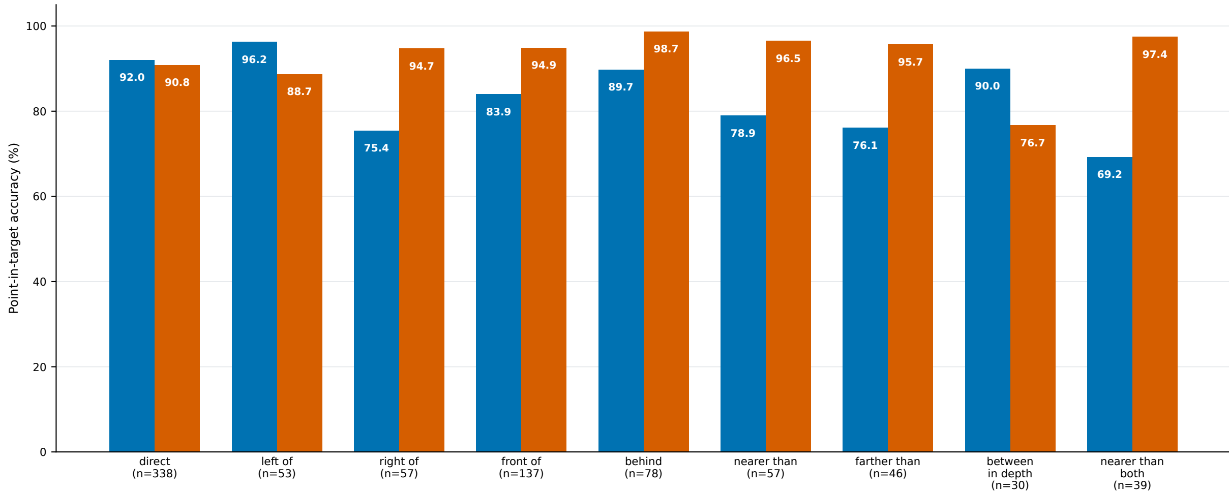
Grounding by relation
