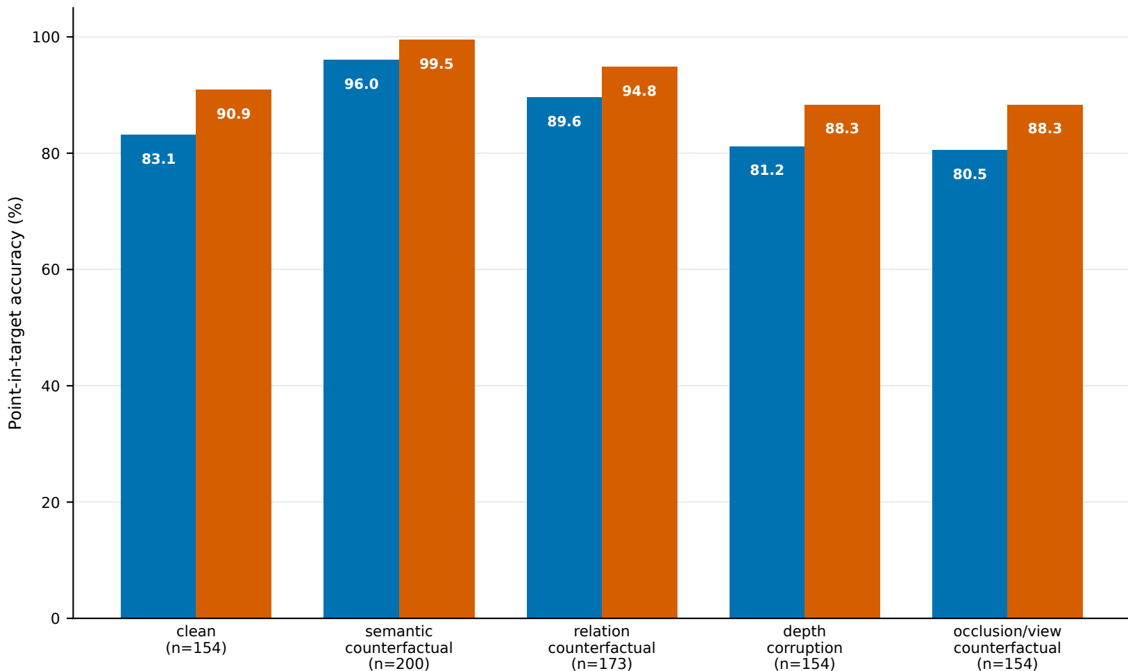
Grounding by Test-IID variant
