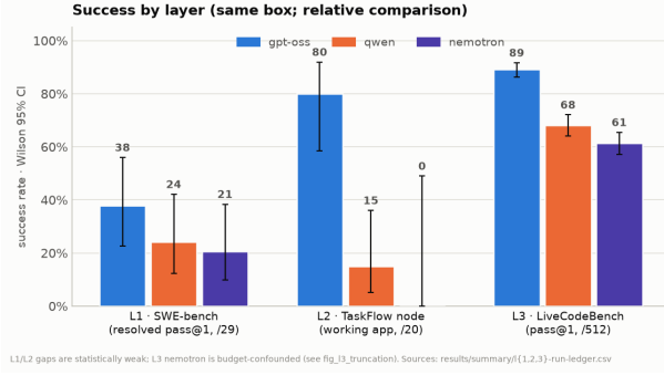
Figure 2: Success by layer for the three configurations, each with a Wilson 95% interval: L1 resolved pass@1, L2 node working-app rate, L3 pass@1. The raw ordering is \text{gpt-oss} \geq \text{qwen} \geq \text{nemotron} , but the L1/L2 separations are weak and the L3 nemotron result is a token-budget artifact (Figure 5).
