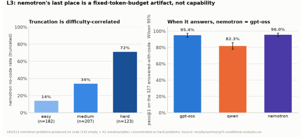
Figure 5: Left: nemotron's no-code (truncation) rate rises with difficulty (easy 14%, medium 34%, hard 72%). Right: on the 327 problems it answers with code—a conditional, easier subset, not comparable to full-set rates—nemotron scores 96.0%, gpt-oss 95.4%, and qwen 82.3%. Much of nemotron's last place in Table 5 reflects truncation under the fixed budget rather than incorrect answers.
