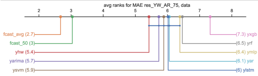
Figure 2: Average ranks for MAE on instance res_YW_AR_75
