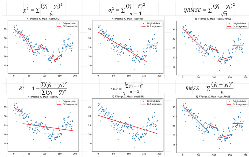
Figure 1. Alternative cost functions
