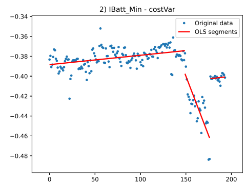
(b) Minimum battery current
