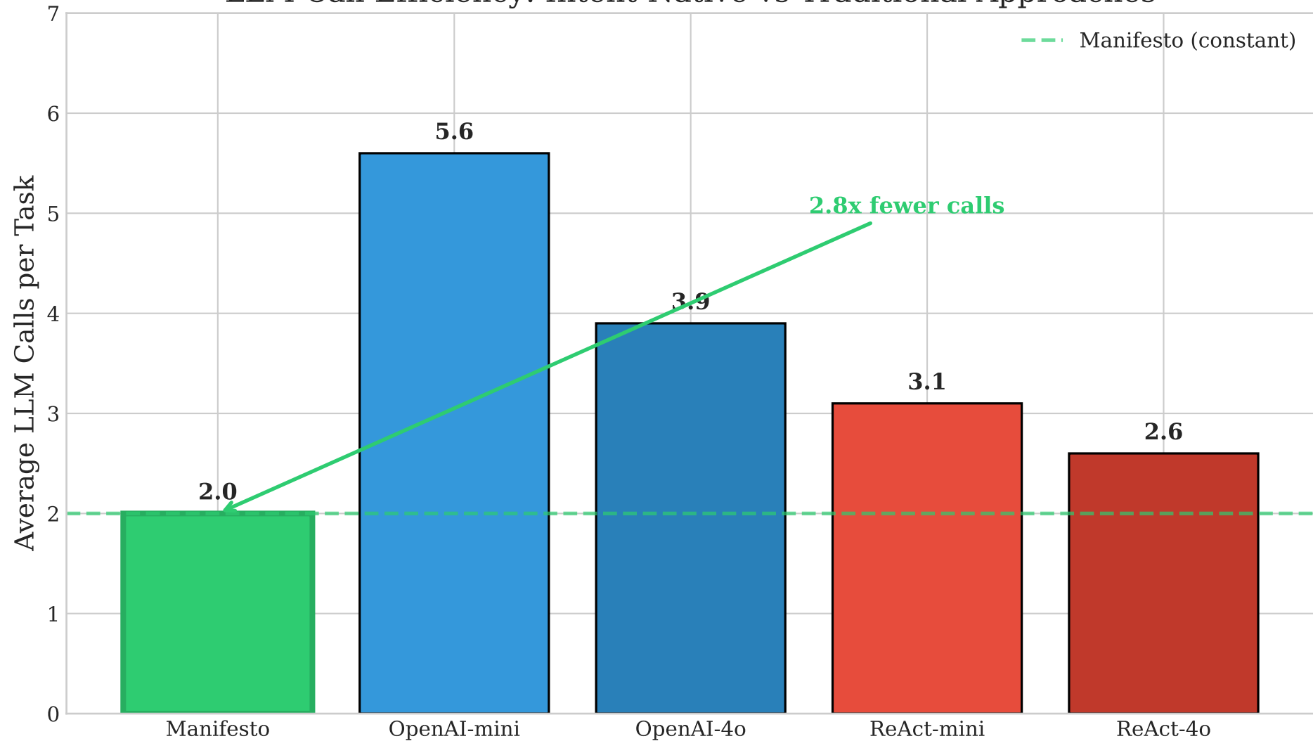
LLM Call Efficiency: Intent-Native vs Traditional Approaches
