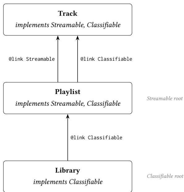
Fig. 1. Composition structure. Arrows show link fields labeled by the delegated interface. Playlist is the root for Streamable dispatch; Library is the root for Classifiable dispatch.
