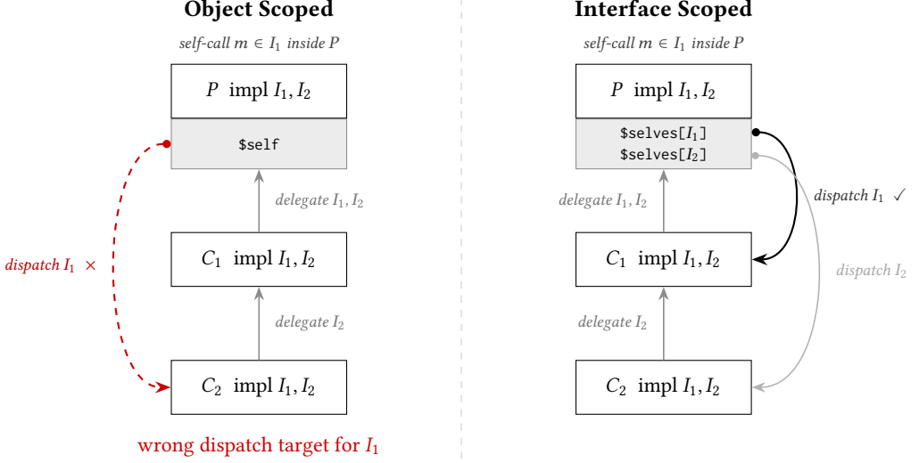
Fig. 3. Object-scoped vs. interface-scoped dispatch. In both panels C_2 (impl I_1, I_2 ) delegates only I_2 to C_1 (impl I_1, I_2 ), which delegates both interfaces to part P . Left : a self-call m() \in I_1 inside P routes through \$self = C_2 , the wrong composite for I_1 . Right : \$selves[I_1] routes to C_1 ; \$selves[I_2] routes to C_2 ; each self-call reaches its correct composite root.
