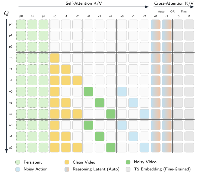
Figure 4: Attention mask of WorldScape Policy 2.0.
