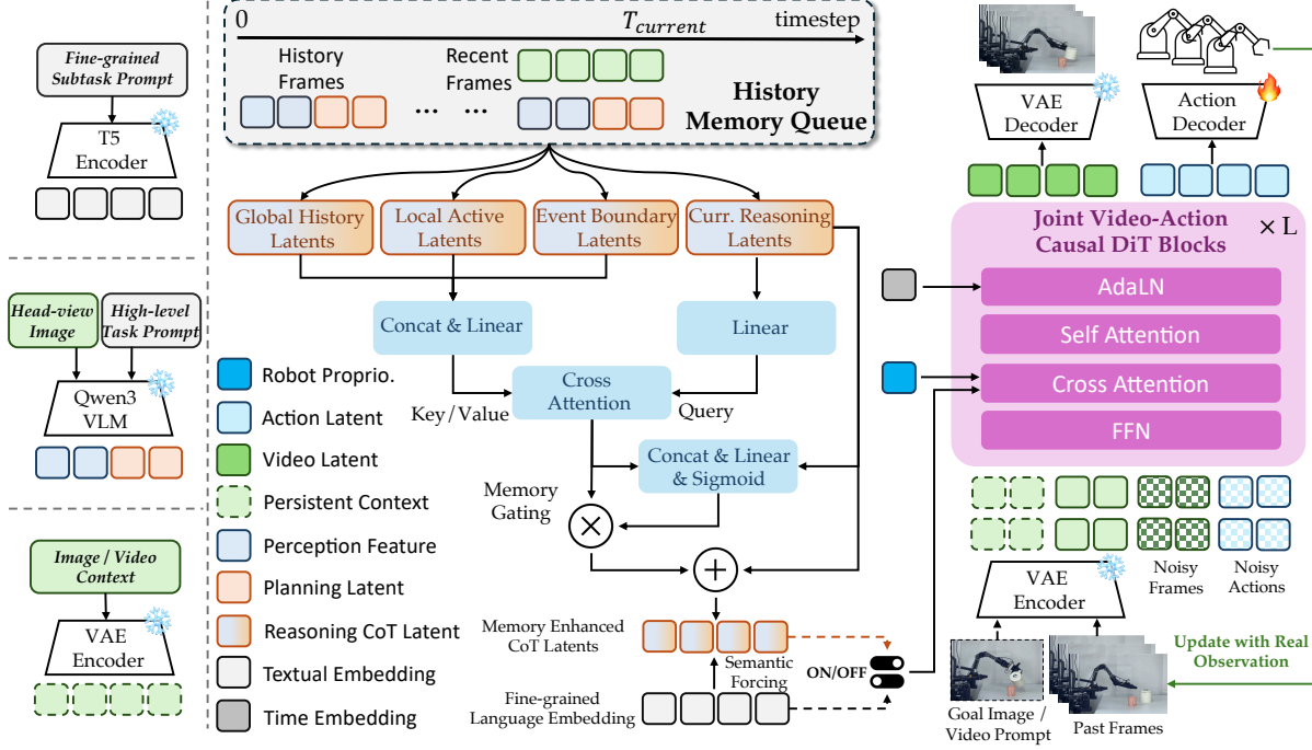
Figure 3: Illustration of Reasoning-Augmented Long Short-Term Memory. Historical VLM outputs form global-history, local-active, and event-boundary memories, which are retrieved and gated to augment the current reasoning tokens; semantic forcing aligns them with subtask semantics. Recent observations and optional visual prompts enter the DiT as causal visual prefill, while memory-enhanced VLM tokens or T5 embeddings condition joint video-action flow prediction according to the interaction mode.
