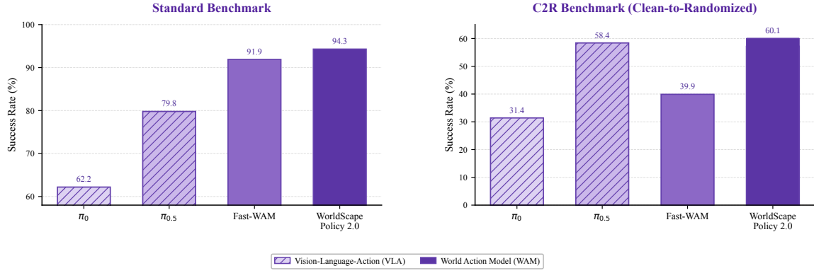
Figure 10: Comparison on the RoboTwin 2.0 standard and C2R benchmarks. The standard benchmark uses clean-plus-randomized training data, whereas C2R trains policies only on clean demonstrations and reports the average success rate across clean and randomized evaluation settings. Hatched bars denote VLA methods, and solid bars denote WAM methods.
