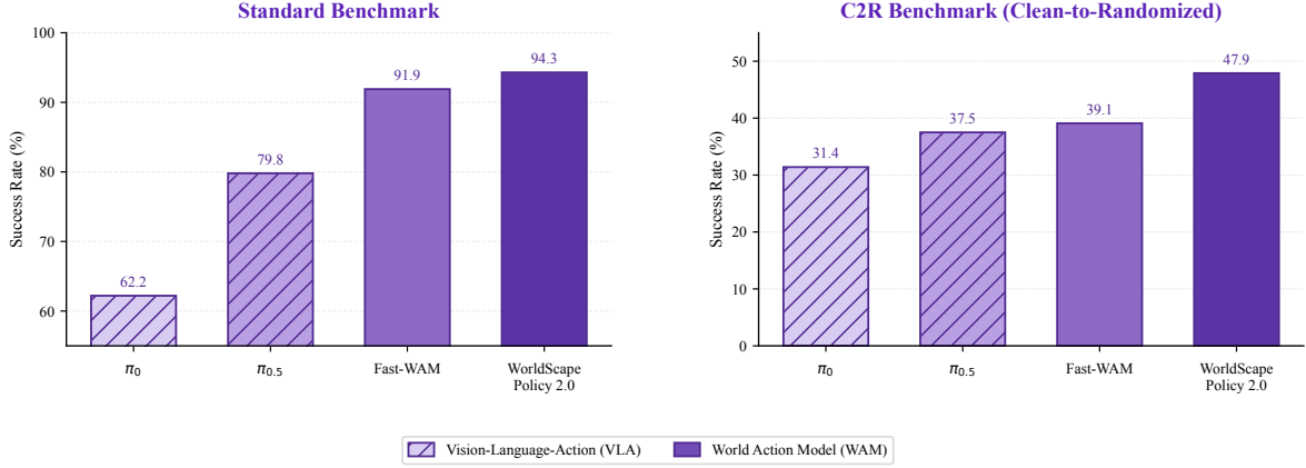
Figure 10: Comparison on the RoboTwin 2.0 standard and C2R benchmarks. The standard benchmark uses clean-plus-randomized training data, whereas C2R trains policies only on clean demonstrations and reports the average success rate across clean and randomized evaluation settings. Hatched bars denote VLA methods, and solid bars denote WAM methods.
