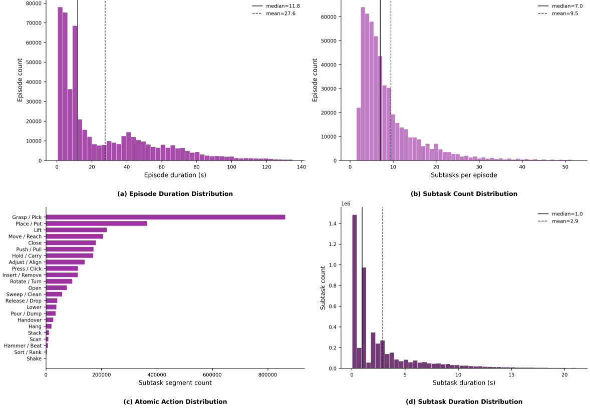
Figure 6: Distribution statistics of ManipEvent-5M. The figure shows the detailed distribution of episode duration, subtask count, atomic actions, and subtask duration across diverse sources from real-world robot data, robot-free data, simulated robot data, and egocentric human data in the constructed ManipEvent-5M.
