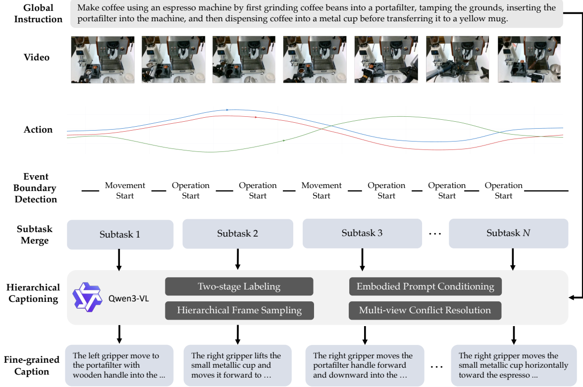
Figure 5: Examples of hierarchical captioning in ManipEvent-5M. The annotation pipeline combines two-stage temporal-semantic labeling, hierarchical episode/event frame sampling, embodied prompt conditioning, and multi-view conflict resolution. The figure shows representative instances that map segmented events to fine-grained captions, complementing the dataset construction pipeline in Fig. 4.
