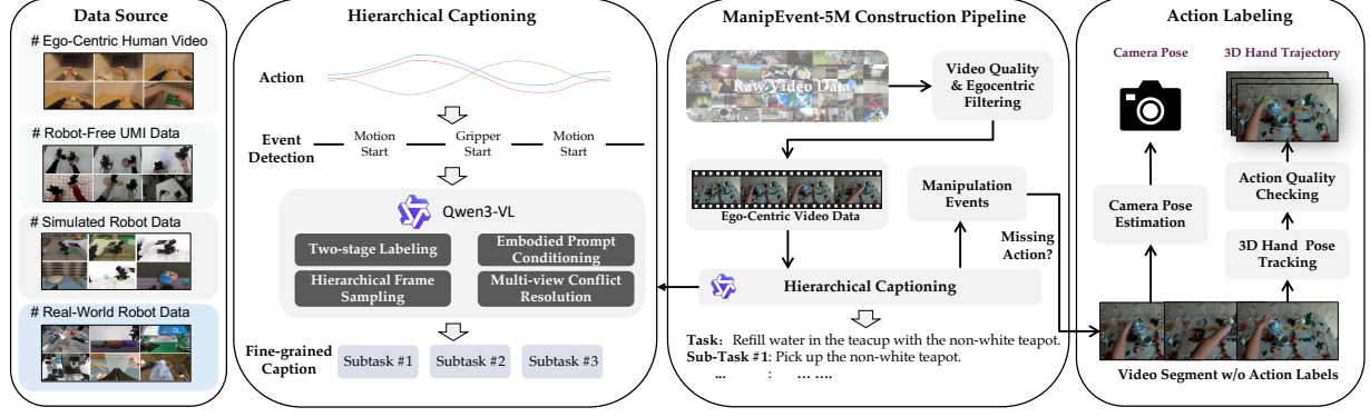
Figure 4: Construction pipeline of ManipEvent-5M. We aggregate heterogeneous manipulation sources, including human-arm ego videos, robot-free UMI data, simulated trajectories, and real-robot demonstrations, and convert them into event-level training samples. Each trajectory is segmented into ordered atomic subgoals and annotated with paired action trajectories, episode-level global instructions, segment-level fine-grained captions, goal-image prompts, and video-context prompts. This event-based multimodal schema supports the event-grounded WAM interface in Fig. 2, enabling fine-grained language grounding, goal-conditioned policy learning, demonstration-conditioned in-context learning, and long-horizon memory mid-training.
