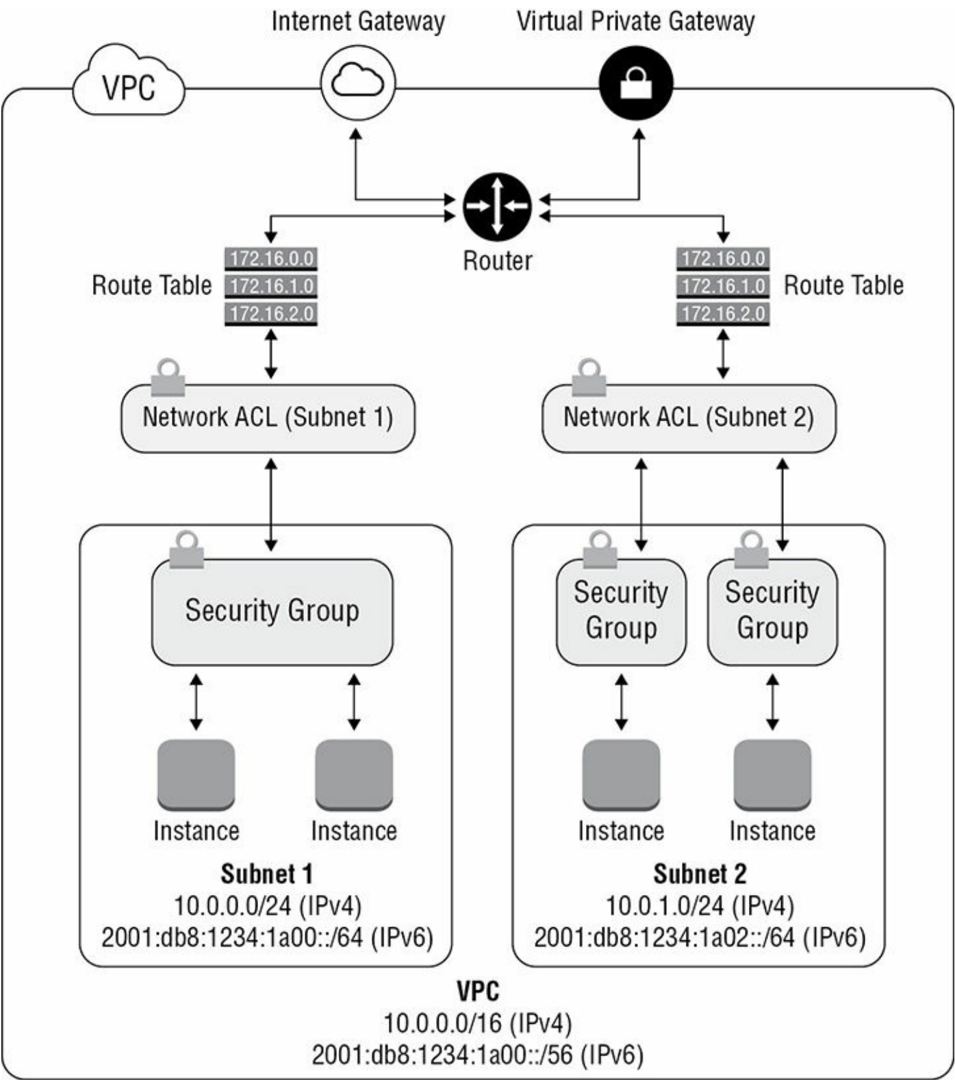
FIGURE 3.6 Flexible network topologies
