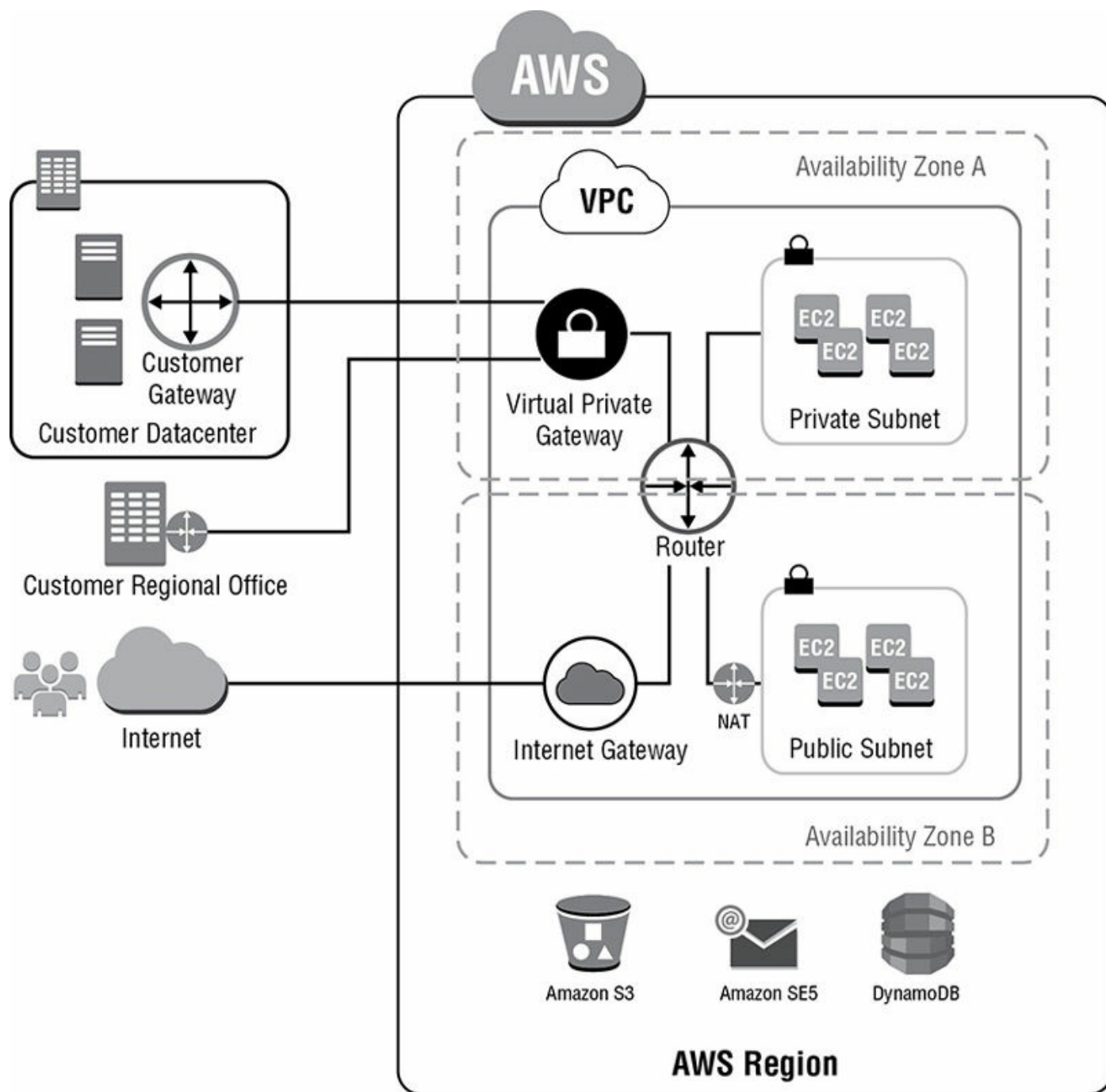
FIGURE 3.5 Amazon VPC network architecture
