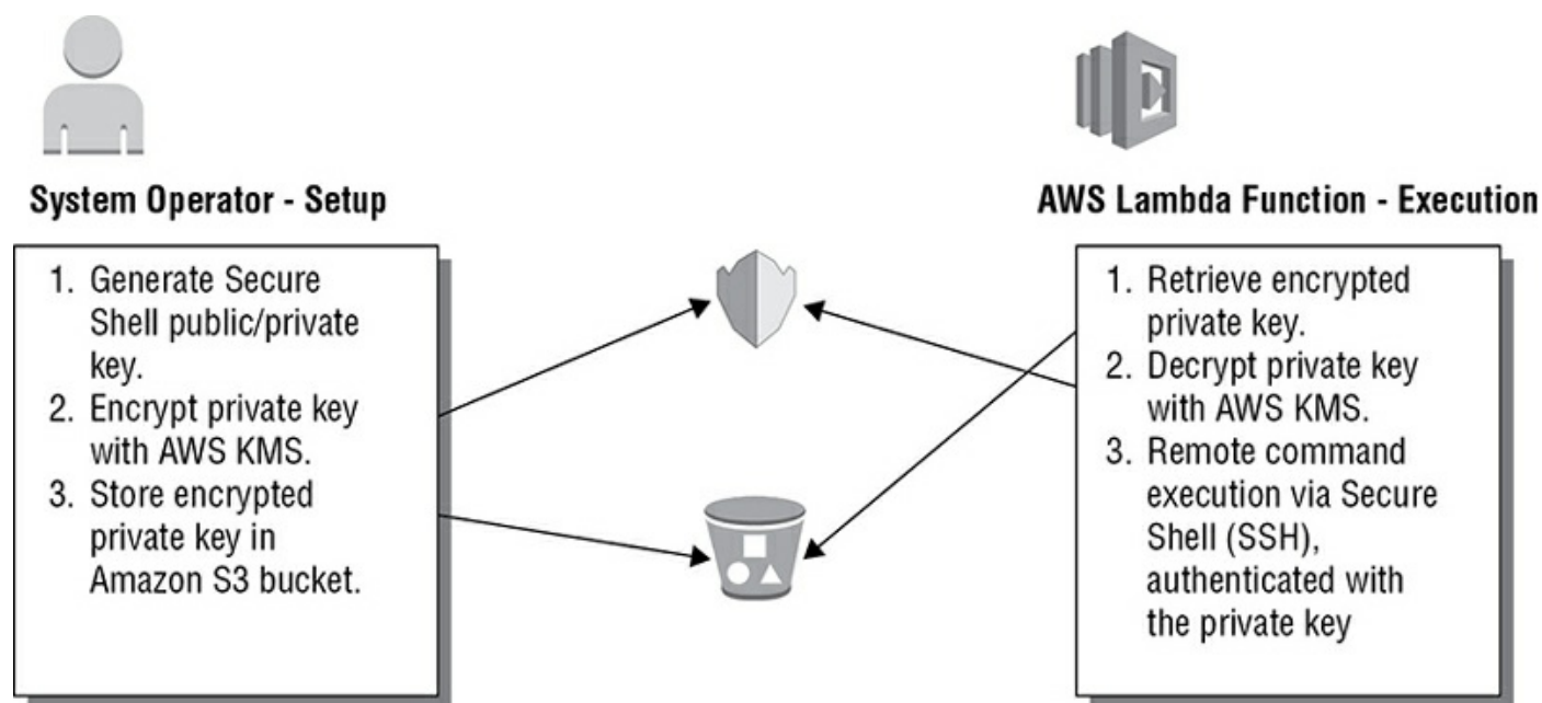
FIGURE 1.2 AWS KMS operations with Lambda
