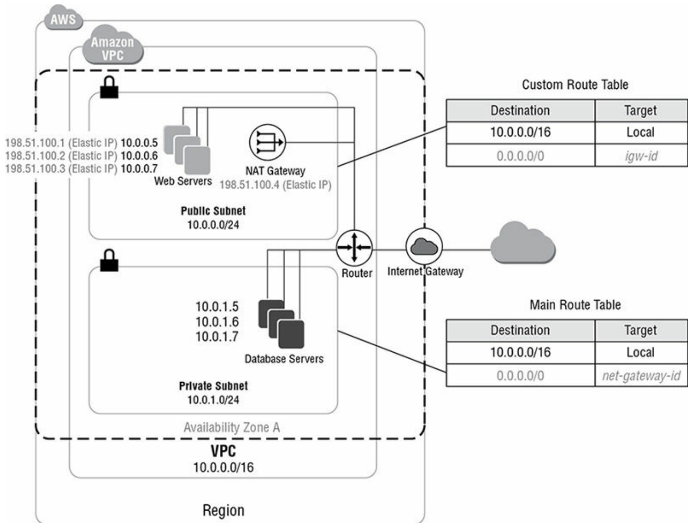
FIGURE 5.4 VPC diagram
