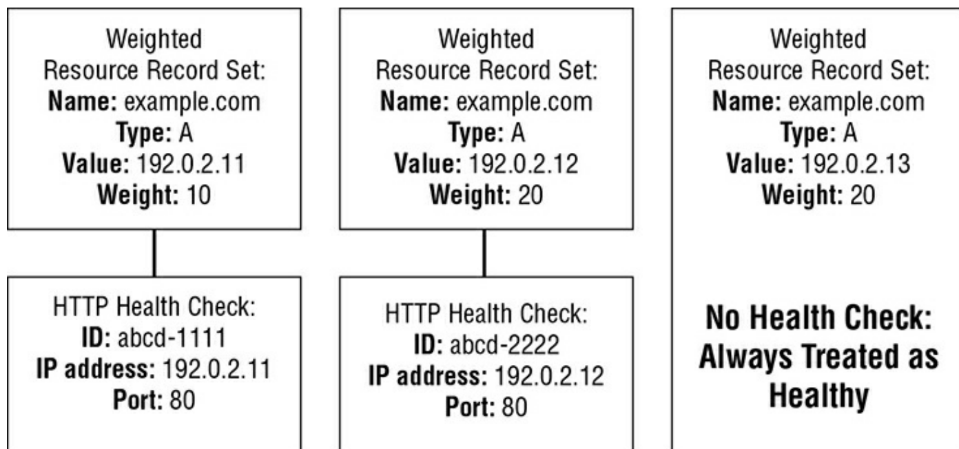
FIGURE 10.8 No health check enabled
