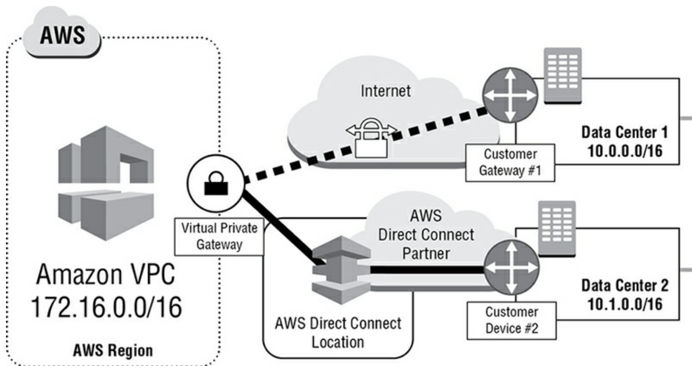
FIGURE 10.13 AWS Direct Connect with backup VPN connection
