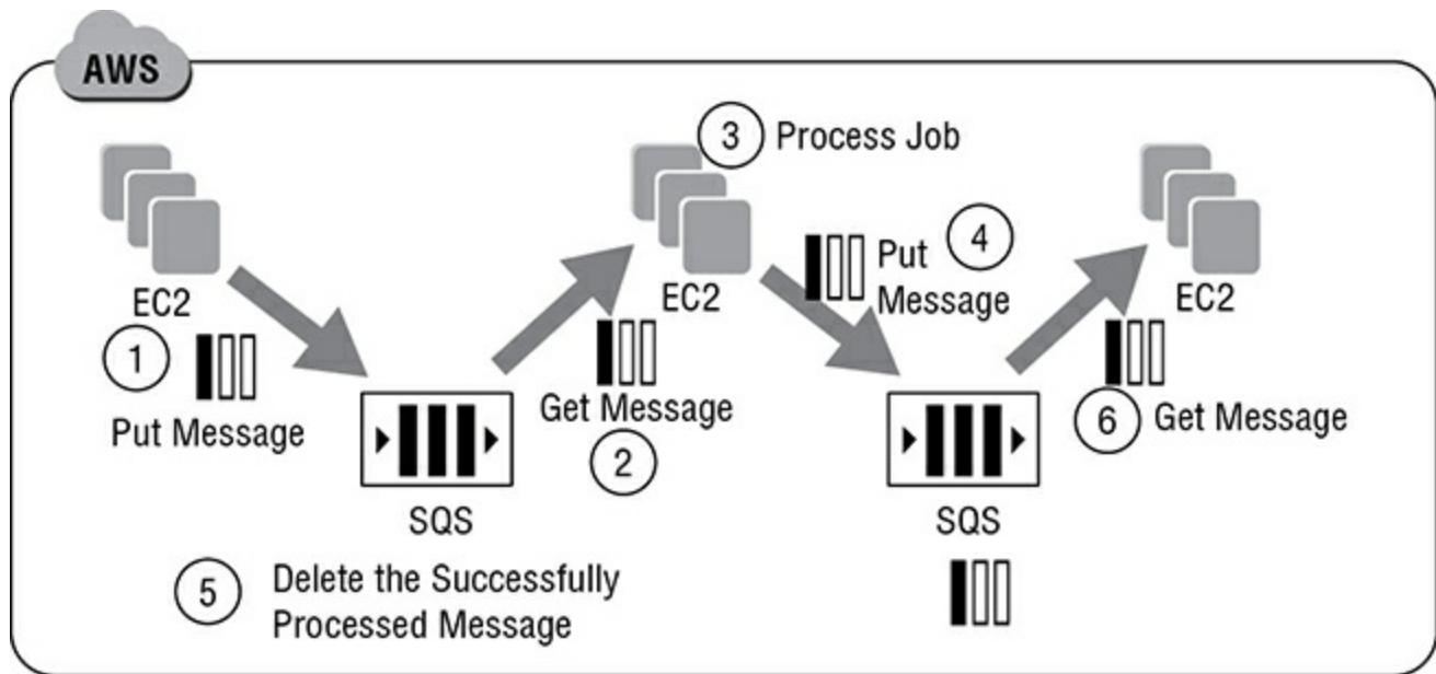
FIGURE 10.1 Demonstrates a queuing chain pattern
