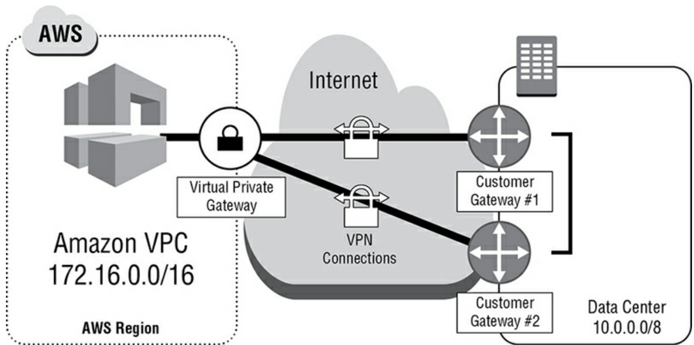
FIGURE 10.11 Redundant active-active VPN connections
