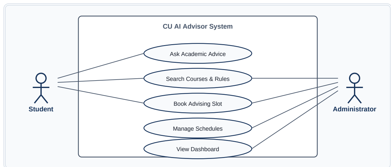
Figure 4.1: UML Use Case Diagram
