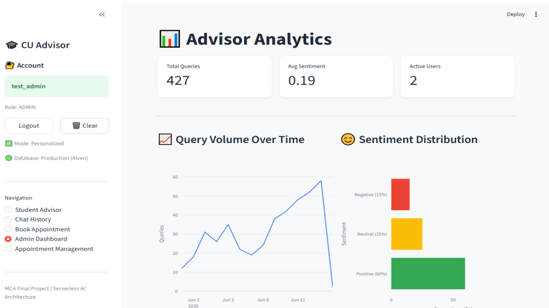
Figure 5.4: Administrator Sentiment & Query Volume Analytics Dashboard
