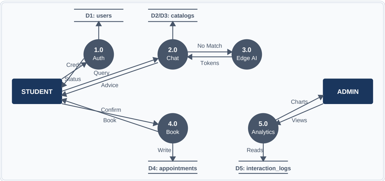
Figure 3.2: DFD Level 1 System Data Flow Diagram
