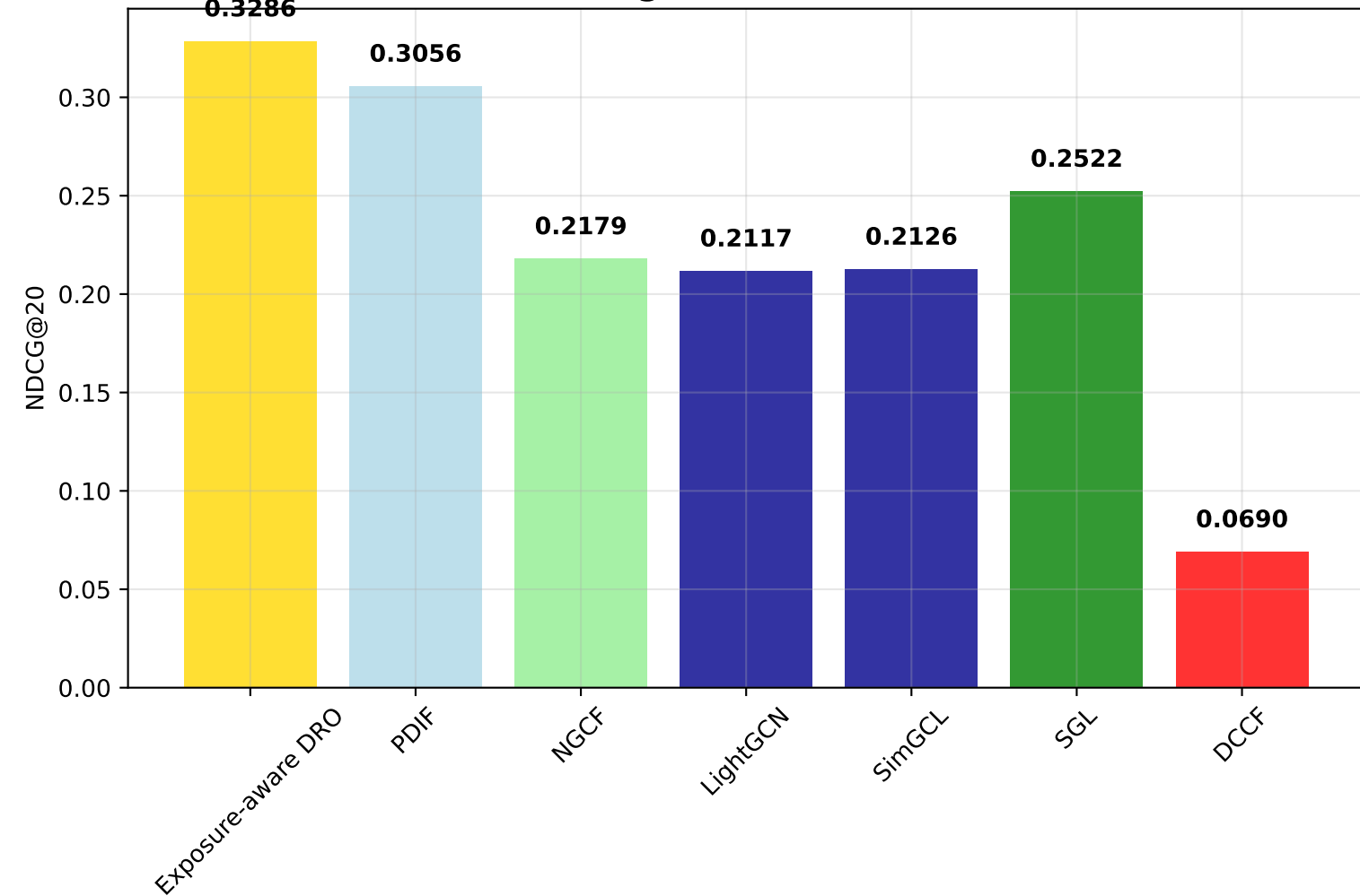
Ranking Quality: NDCG@20 (Higher = Better)
