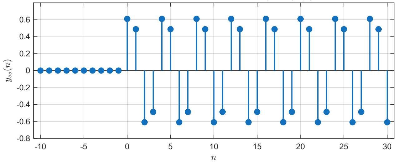
Steady State Response output for \cos(0.5\pi n)u(n)
