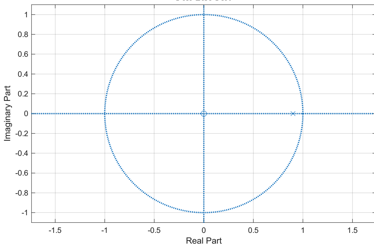
Pole-Zero Plot
