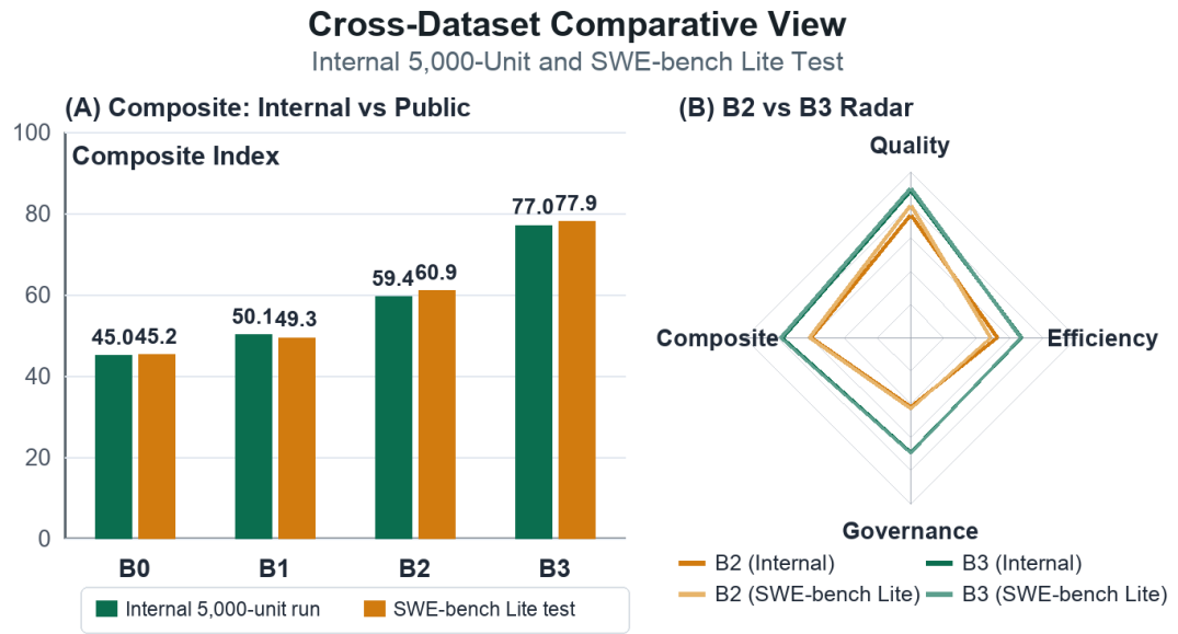
Fig. 9. Cross-input sensitivity view. Panel (A) reports scoring-model B0–B3 composite scores for internal generated units and public issue text. Panel (B) overlays the corresponding B2/B3 profiles. No patches or benchmark tests are executed.
