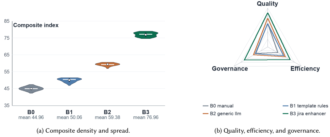
Fig. 8. Two diagnostics from the 5,000-unit stress test. Panel (a) shows density, interquartile range, median, and mean. Panel (b) shows the mean component indices. Both panels audit the scoring model. They do not report observed comparative performance.
