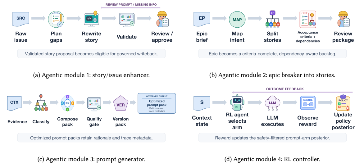
Fig. 3. Modular agent architecture: story/issue enhancement, epic-to-story decomposition, prompt-pack creation, and RL-based policy control. The panels expose agent boundaries hidden in the top-level architecture.
