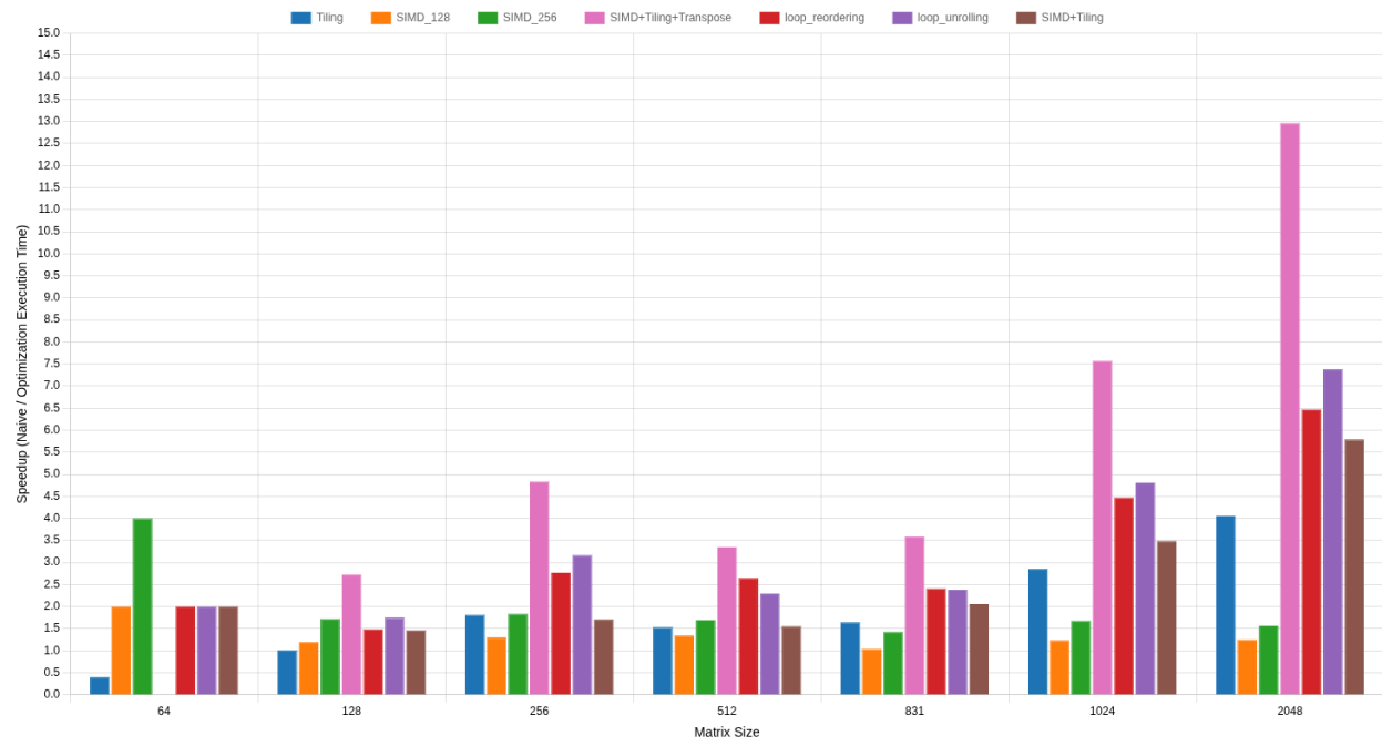
Speedup vs. Matrix Size (64 to 2048) for Different Optimizations
