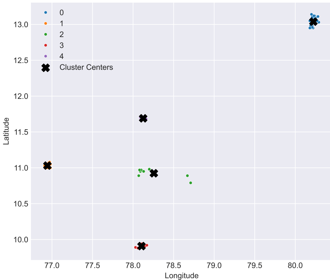
K-Means Violation Hotspot Clusters (5 Zones)
