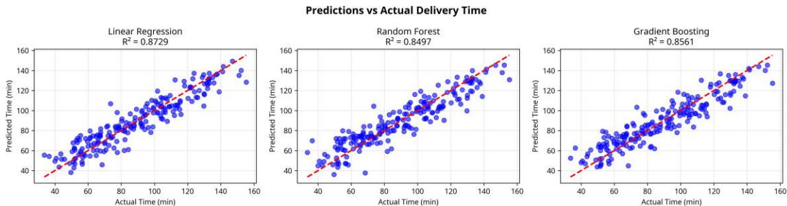
Figure 3: Predictions vs Actual Delivery Time for all models
