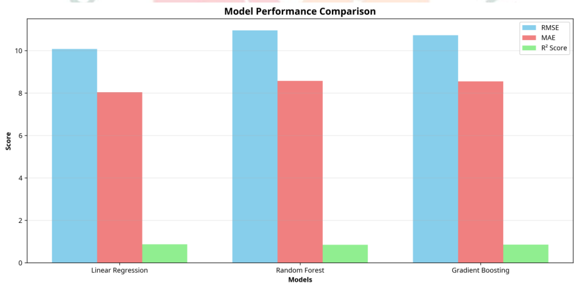
Figure 2: Model Performance Comparison (RMSE, MAE, R² Score)
