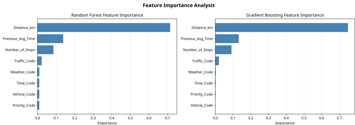
Figure 4: Feature Importance Analysis for Random Forest and Gradient Boosting
