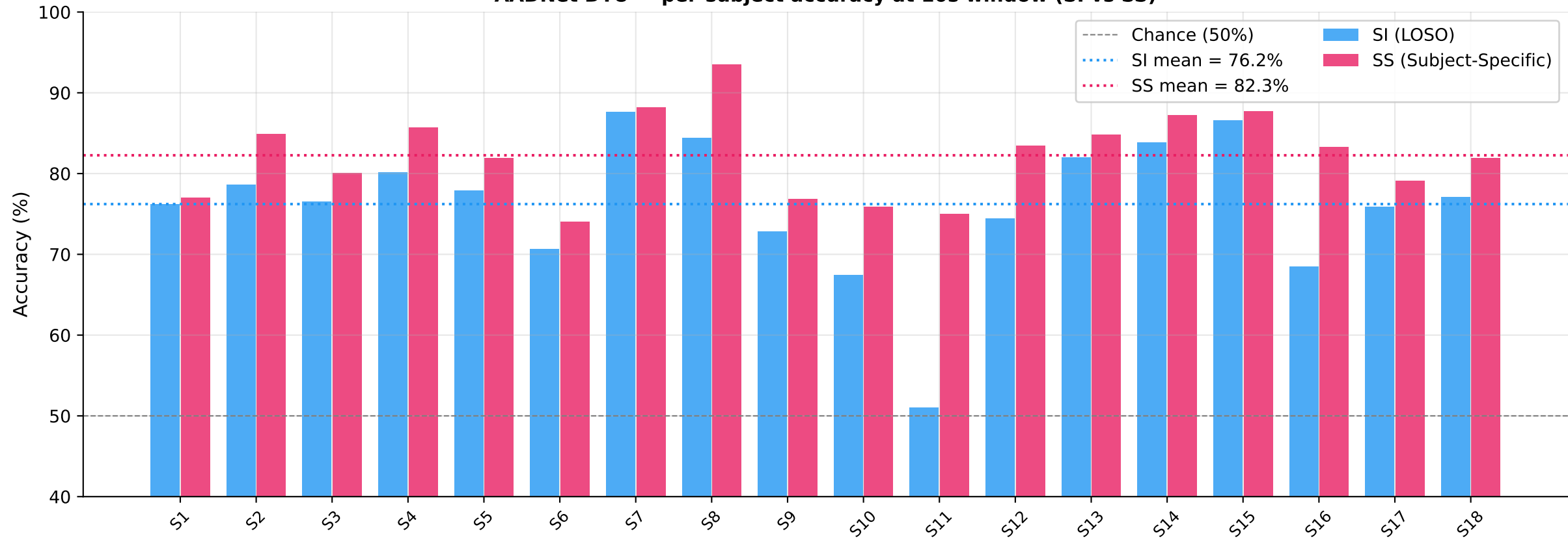
AADNet DTU — per-subject accuracy at 10s window (SI vs SS)
