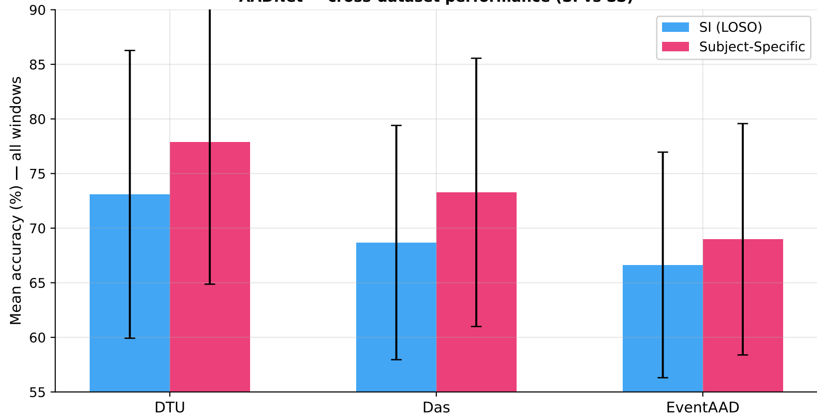
AADNet — cross-dataset performance (SI vs SS)
