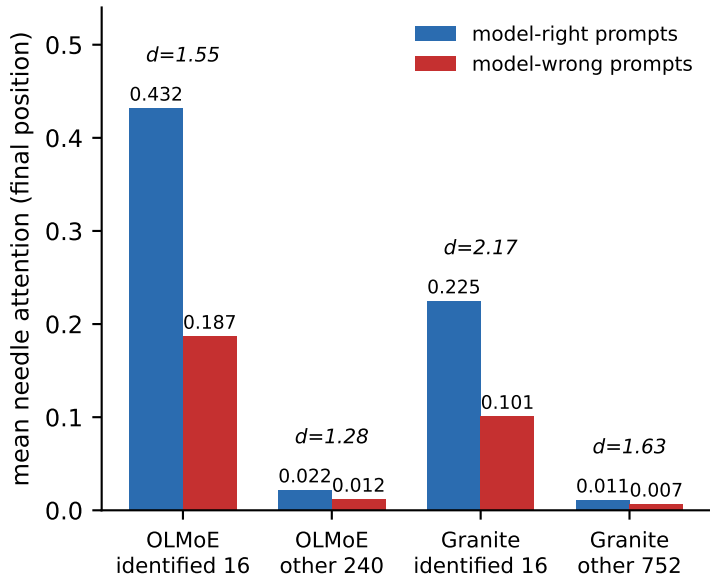
(b) Collapse is localized (3,840 tokens)
