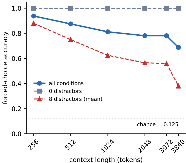
(a) Length degradation, OLMoE
