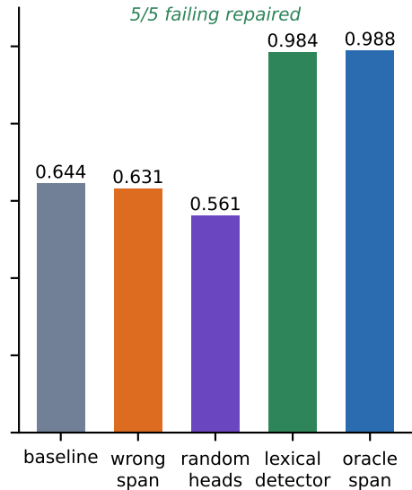
Granite hard set (n=16)
