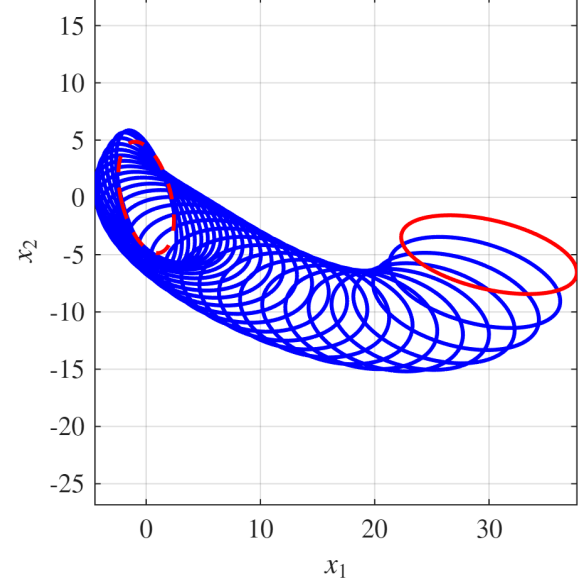
(b) Square root QR covariance steering result
