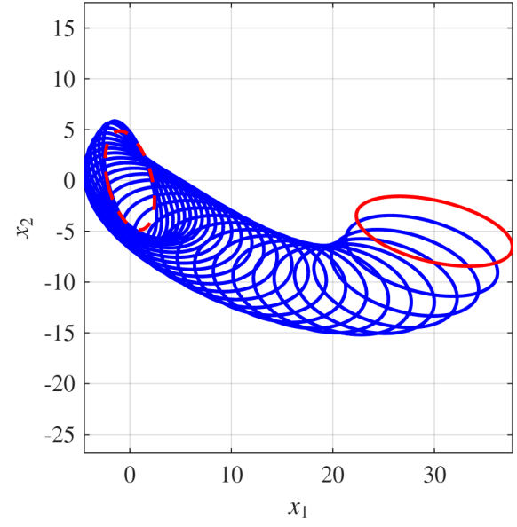
(b) Square root QR covariance steering result
