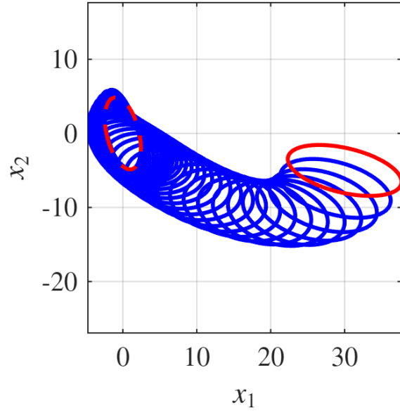
(a) Full covariance steering result
