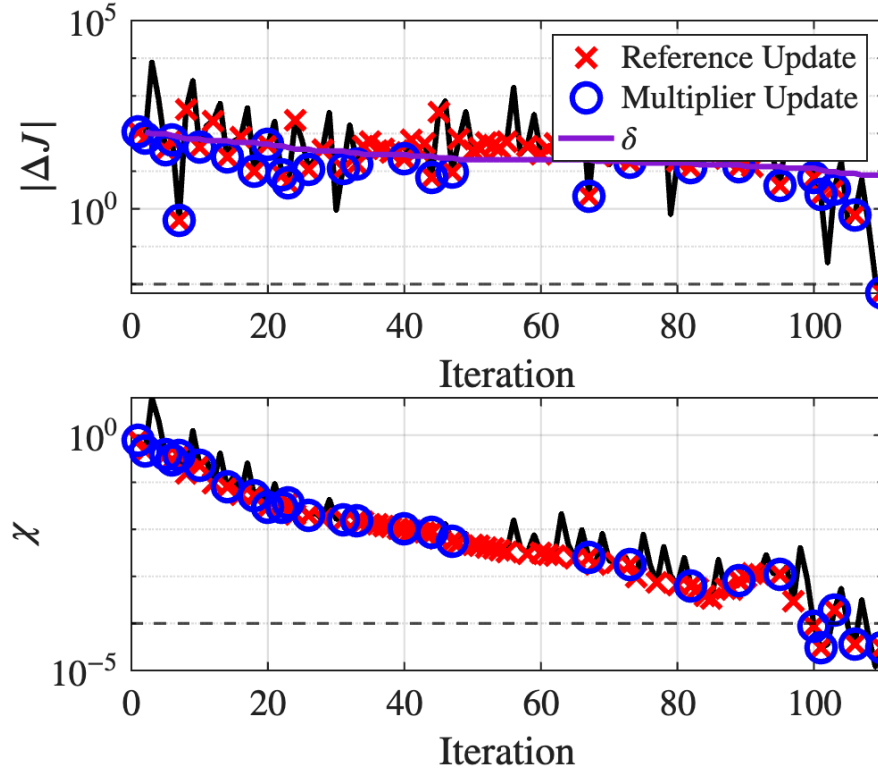
Figure 7: Convergence history of the SCvx* algorithm for the proposed method
