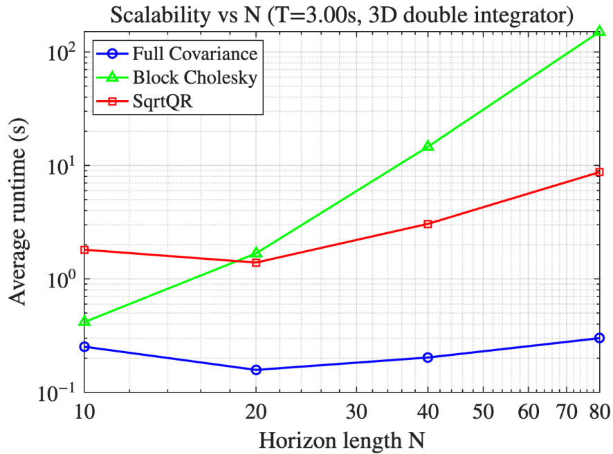
Figure 5: Comparison of solutions times between full covariance, block cholesky, and square root QR covariance steering methods
