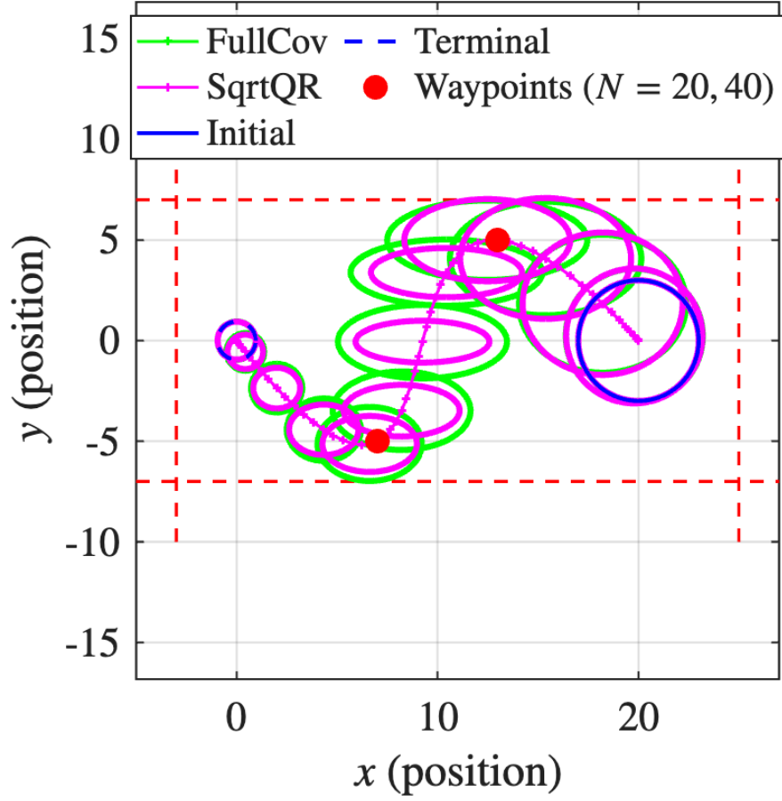
Figure 6: Example trajectory for quadrotor 2D path planning, solved using FullCov and SqrtQR methods
