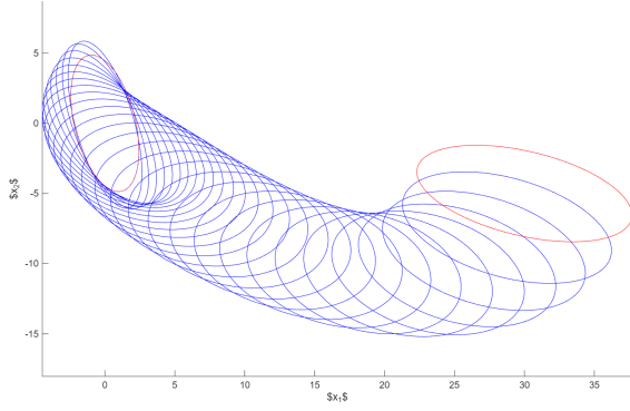
(a) Full covariance steering result
