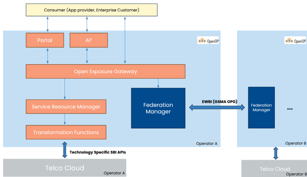
Figure 2.8: ETSI OpenOP Release 1 architecture [29]
