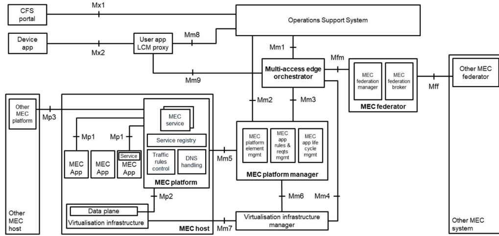
Figure 2.7: ETSI MEC federation architecture variant [26]
