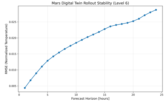
Figure 2. Rollout stability over 24 forecast hours. RMSE of normalized temperature increases monotonically from \sim 0.004 to \sim 0.029 without divergence, demonstrating the model’s ability to maintain physically coherent forecasts for a full Martian sol.
