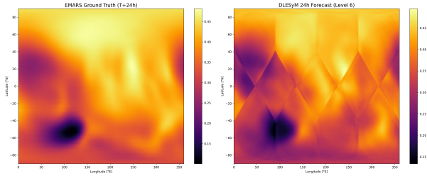
Figure 3. 24-hour rollout comparison. Left: EMARS ground truth at T+24 h. Right: HEALPix U-Net prediction after 24 recursive steps. The model maintains realistic large-scale structures including the polar vortex and equatorial gradients, though faint HEALPix face-boundary artifacts emerge at long lead times.
