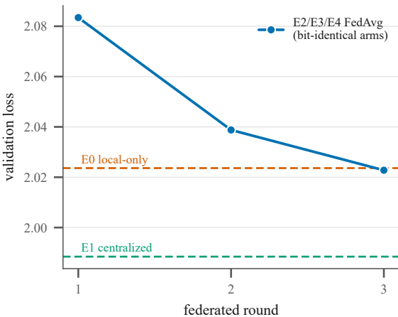
SmolLM2-360M
