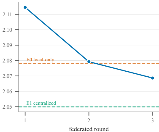
Qwen2.5-0.5B
