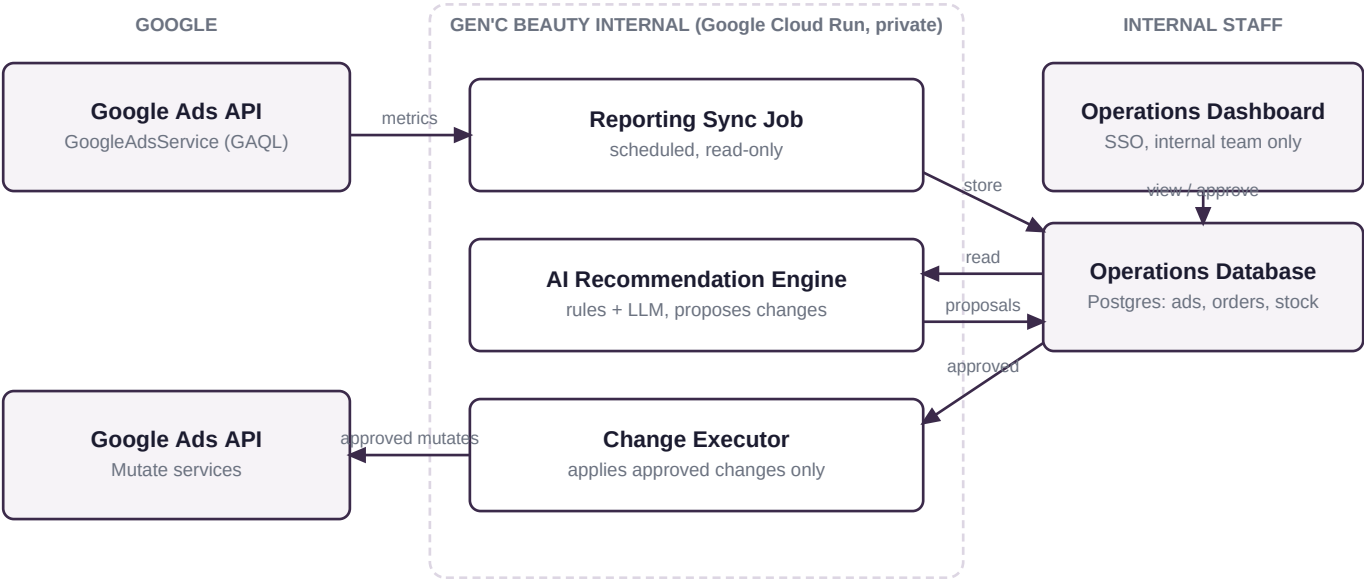
Figure 1. High-level data flow. All API traffic originates from one private service; no external party has access.
