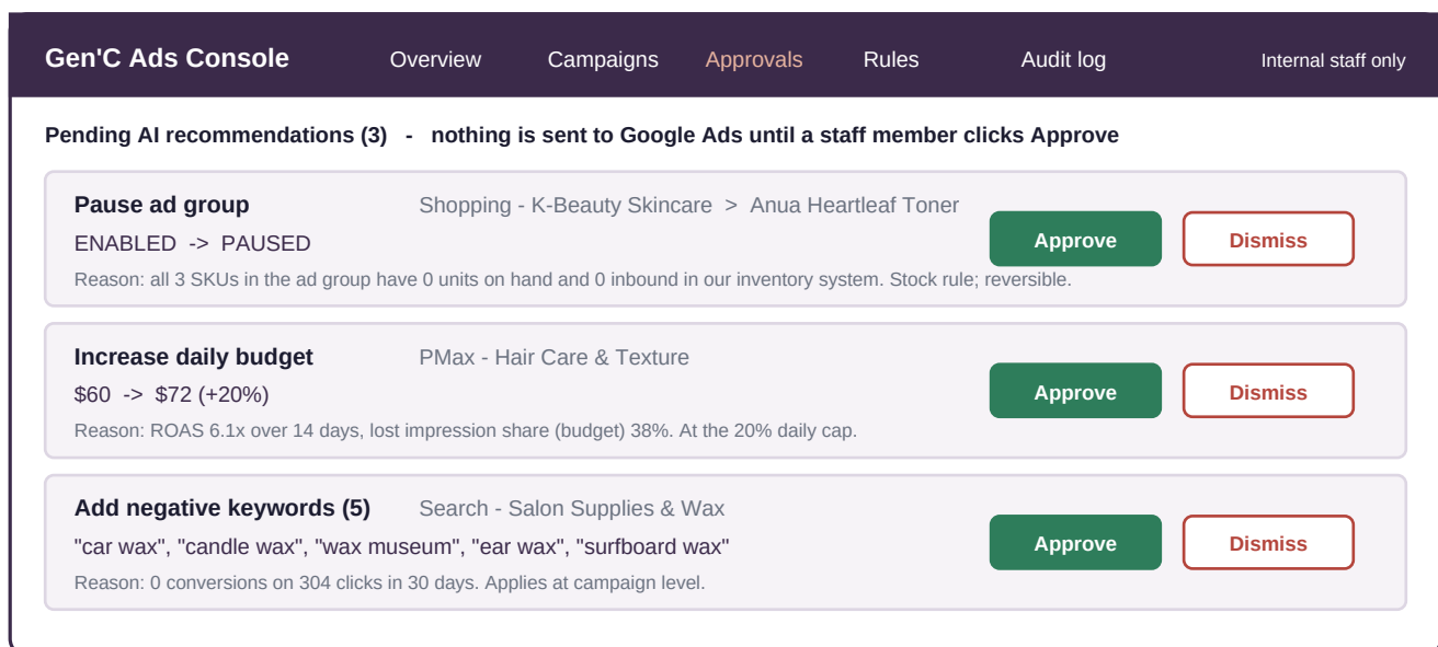
Figure 3. Approval queue (mockup). Each card maps to one mutate operation and is logged with approver, time and before/after values.
