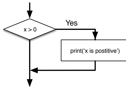
Figure 3.1: If Logic
