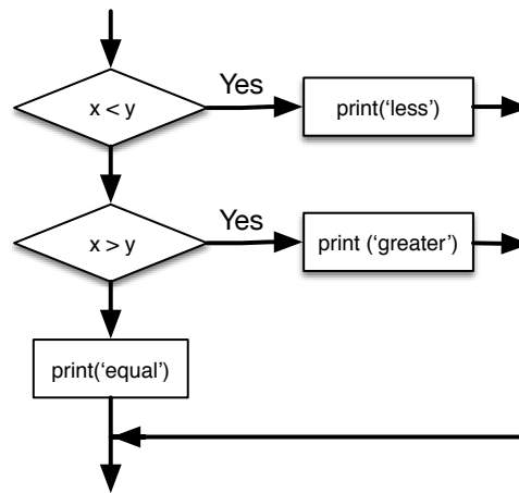
Figure 3.3: If-Then-ElseIf Logic
