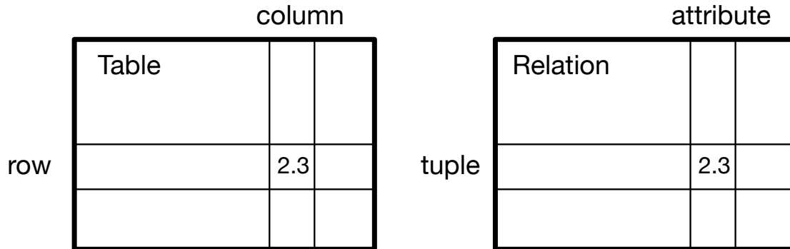
Figure 15.1: Relational Databases
