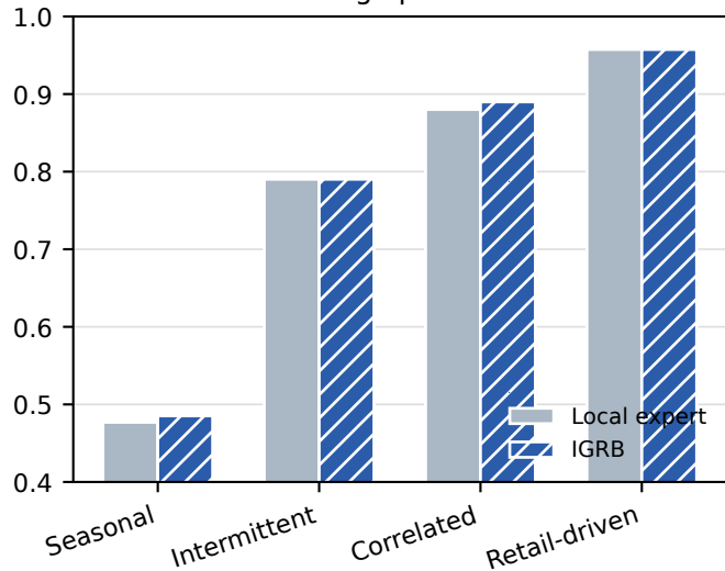
Average precision
