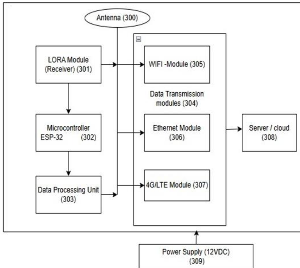
FIG. 3: BLOCK DIAGRAM OF LORA RECEIVER
