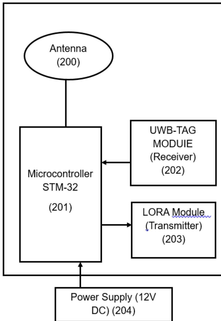
FIG. 2: BLOCK DIAGRAM OF LORA TRANSMITTER
