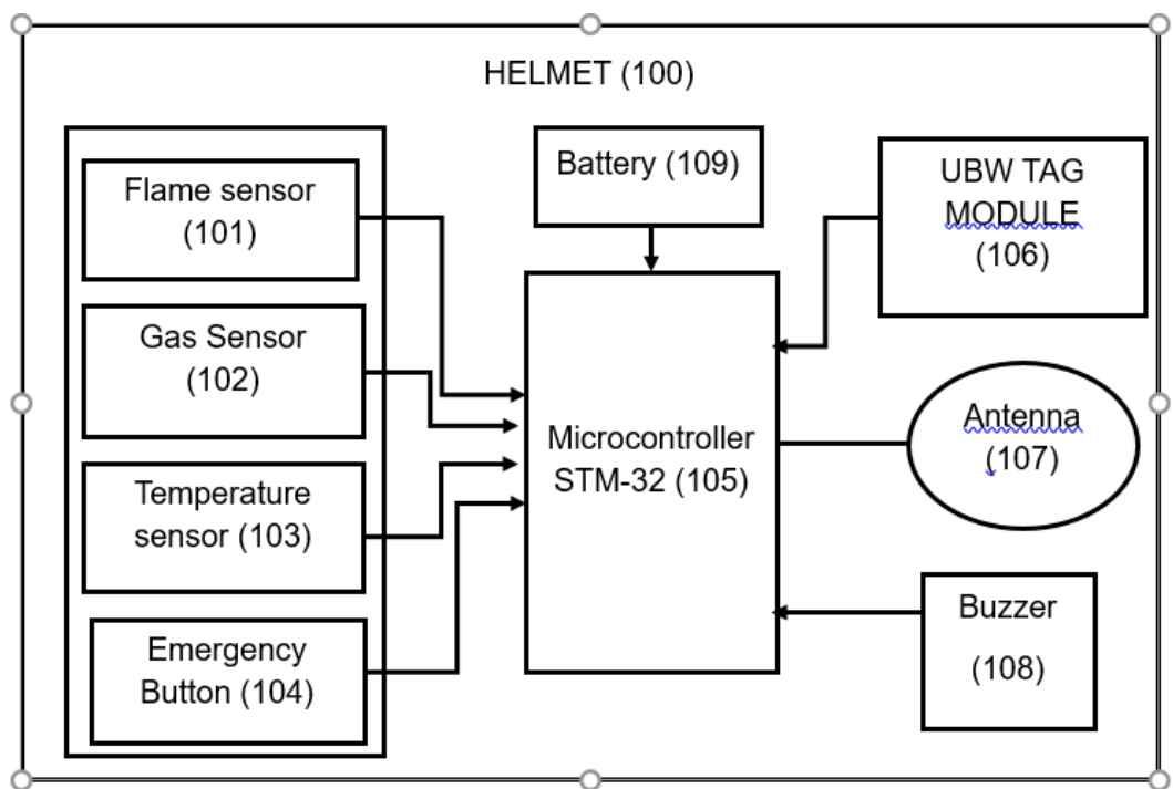
FIG. 1: BLOCK DIAGRAM OF A SMART HELMET
