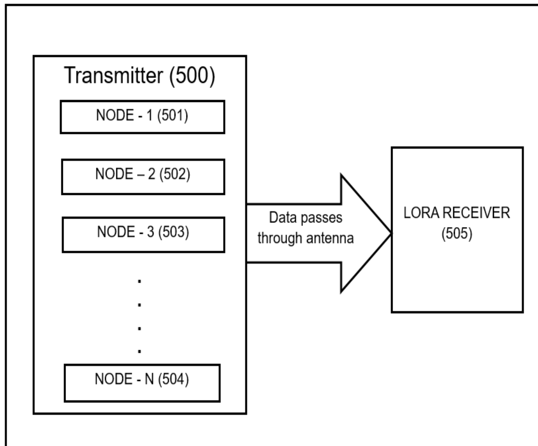
FIG. 5: BLOCK DIAGRAM OF TUNNEL GATEWAY
