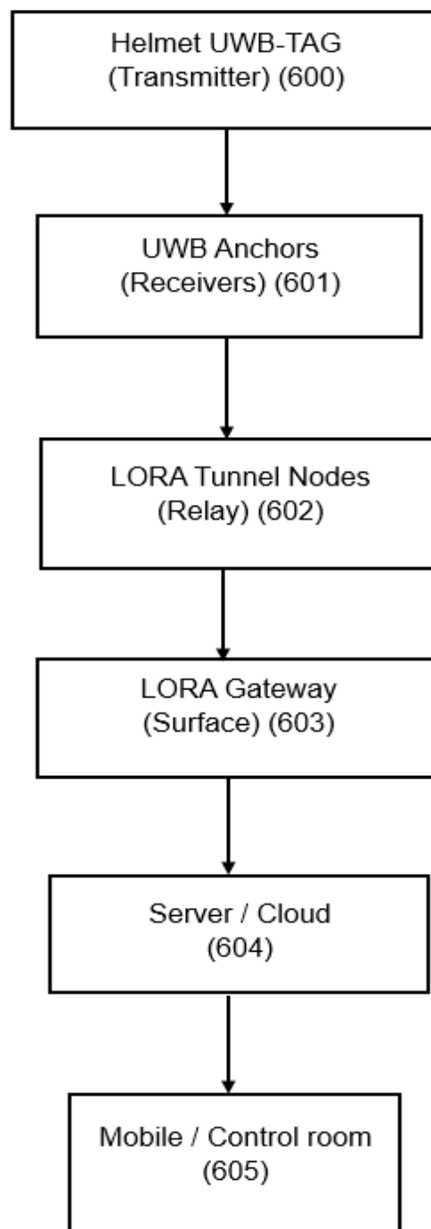
FIG. 6: COMMUNICATION FLOW
