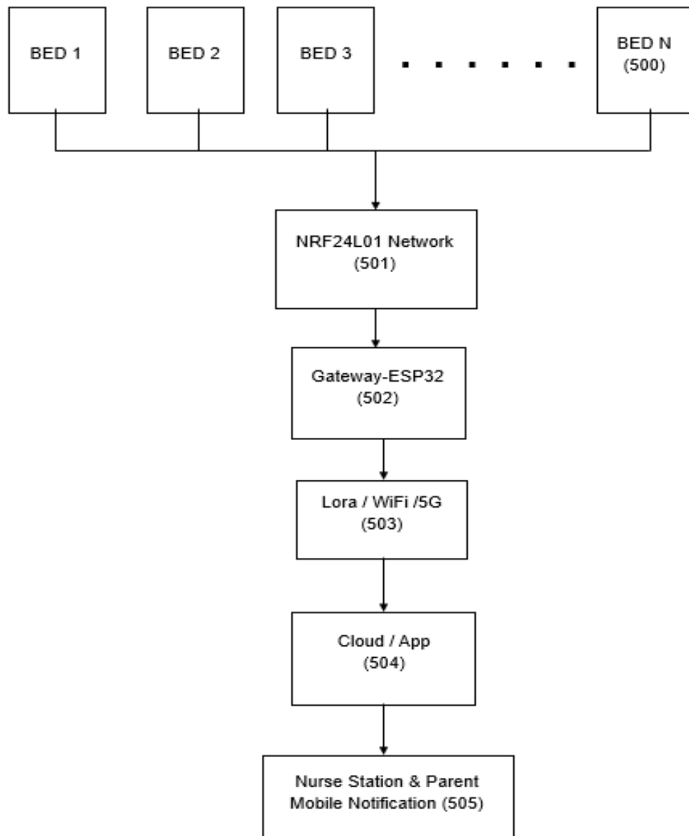
FIG. 5: COMMUNICATION FLOW
