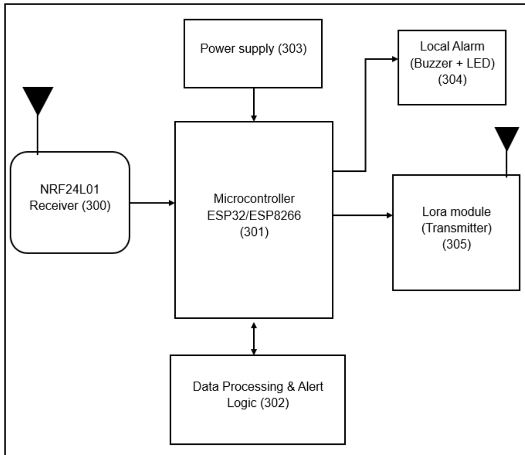
FIG. 3: BLOCK DIAGRAM OF ICU CENTRAL UNIT
