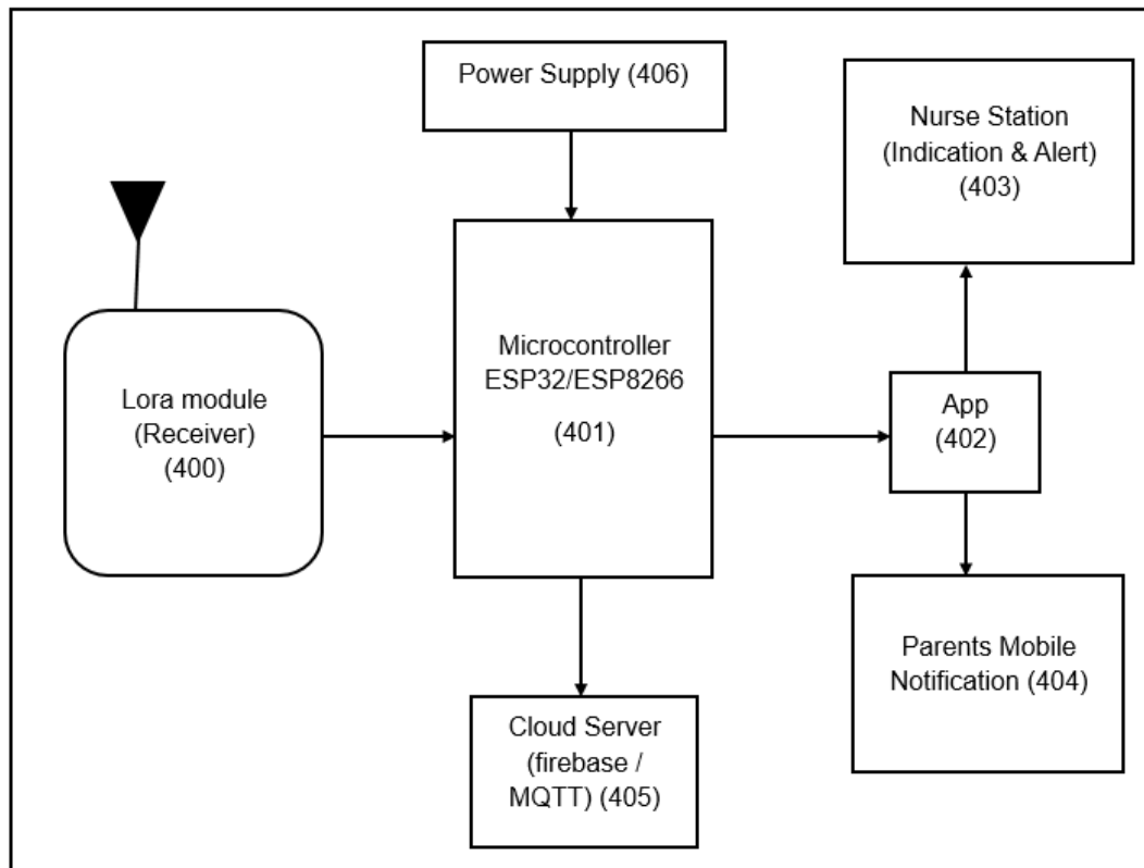
FIG. 4: BLOCK DIAGRAM OF ICU RECEIVER UNIT
