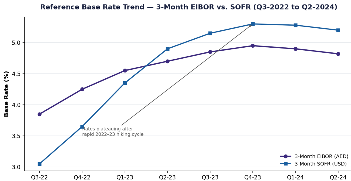
Figure 3.1 — 3-month EIBOR vs. SOFR trend, Q3-2022 to Q2-2024.
