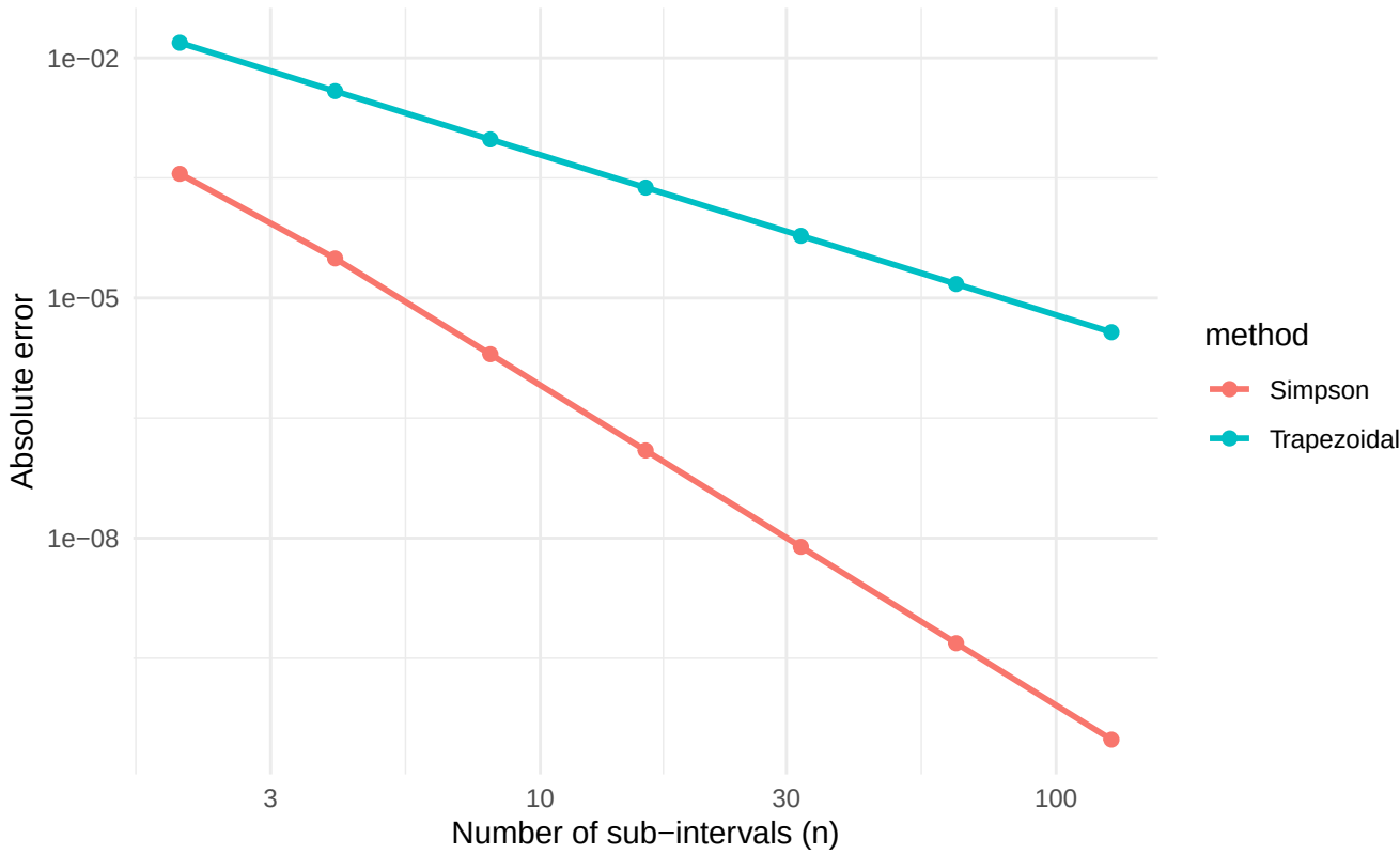
Quadrature error vs. number of sub-intervals (log-log scale)
