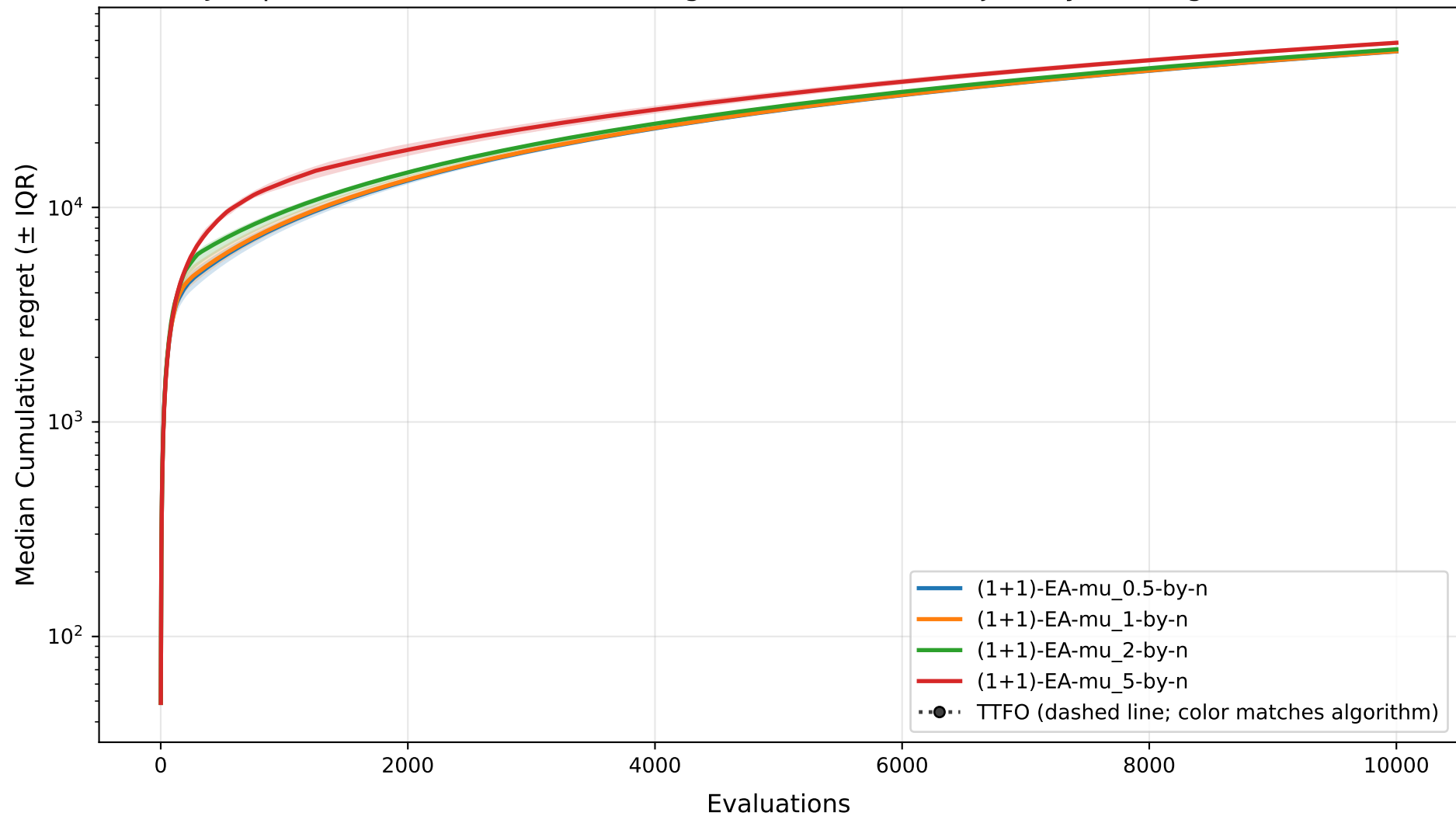
Jump-k5 - n=100: Cumulative Regret (incumbent) Trajectory at Budget=10000
