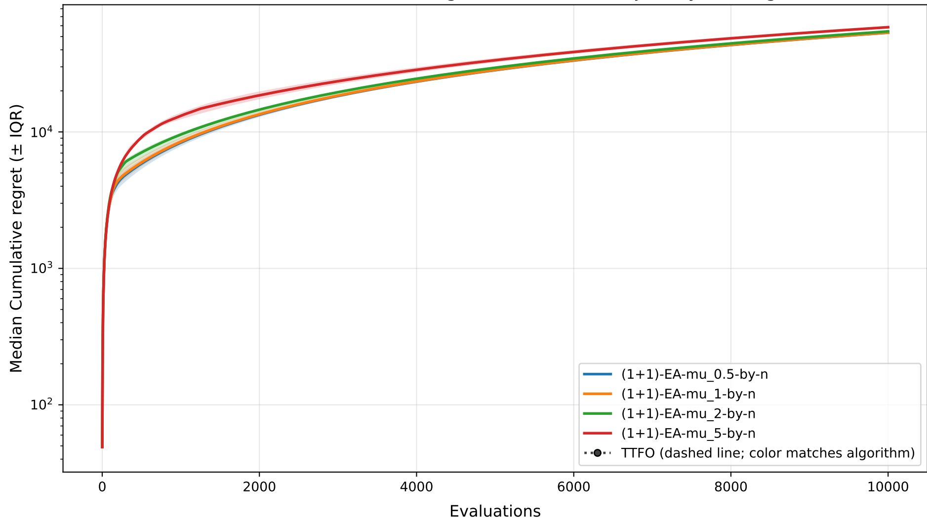
Plateau-k5 - n=100: Cumulative Regret (incumbent) Trajectory at Budget=10000
