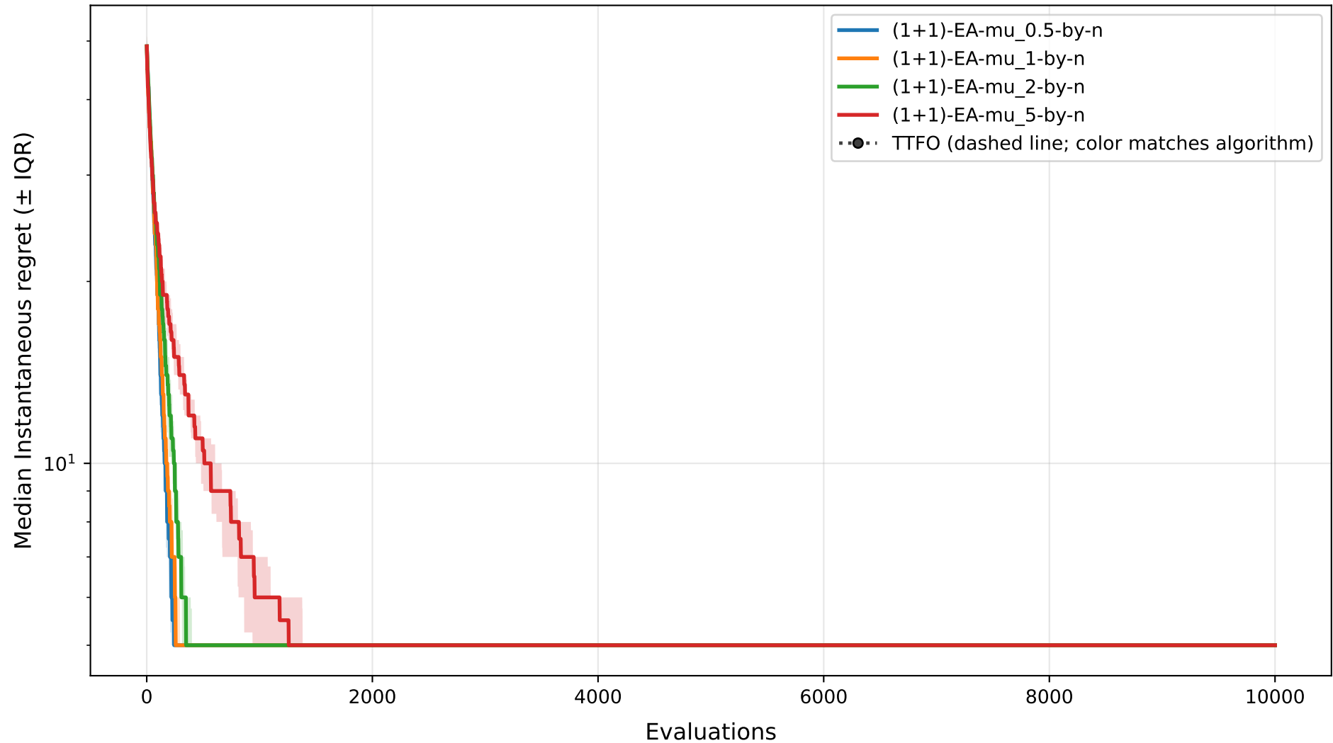
Plateau-k5 - n=100: Instantaneous Regret (incumbent) Trajectory at Budget=10000
