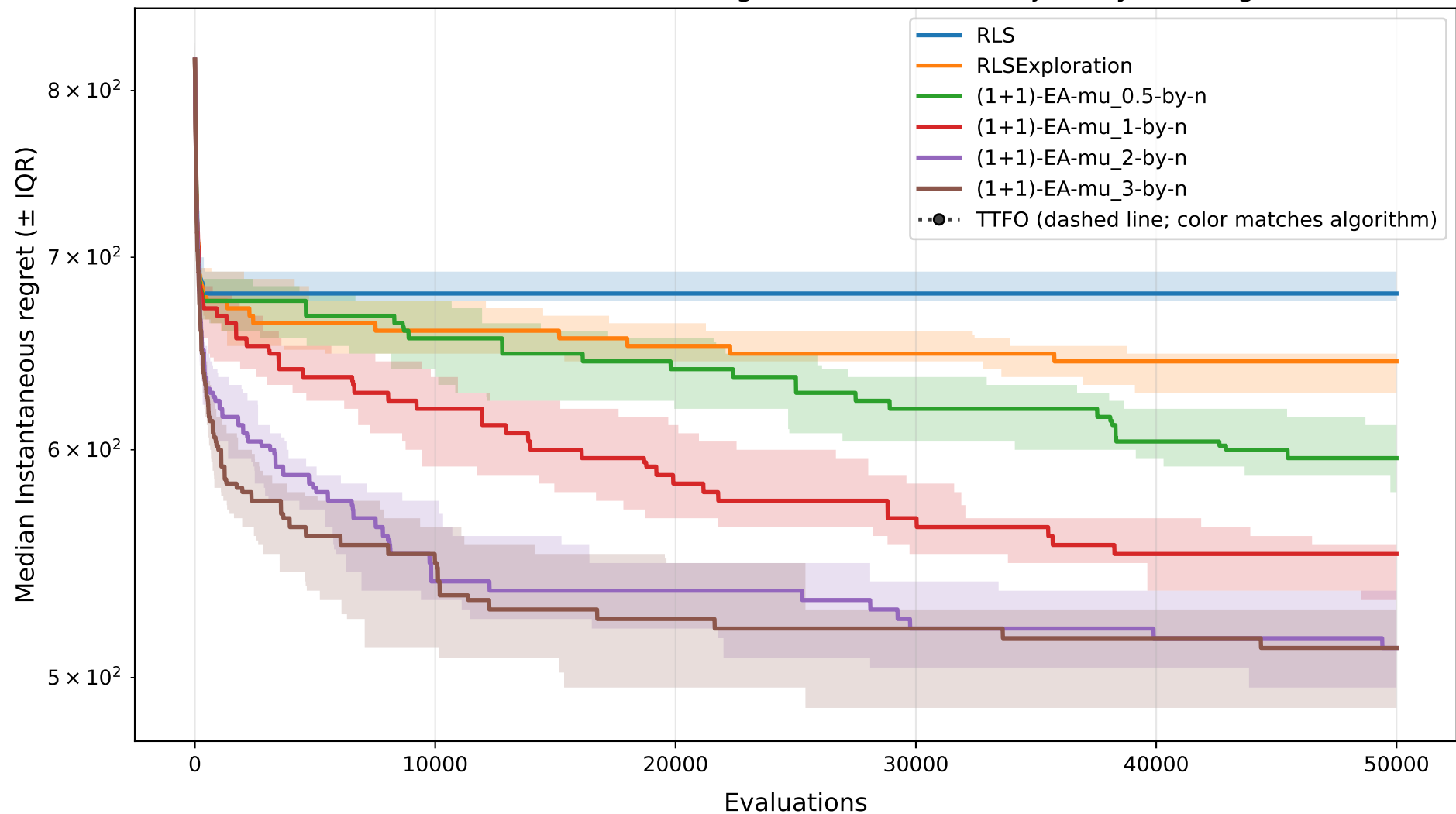
HIFF-n128 - n=128: Instantaneous Regret (incumbent) Trajectory at Budget=50000
