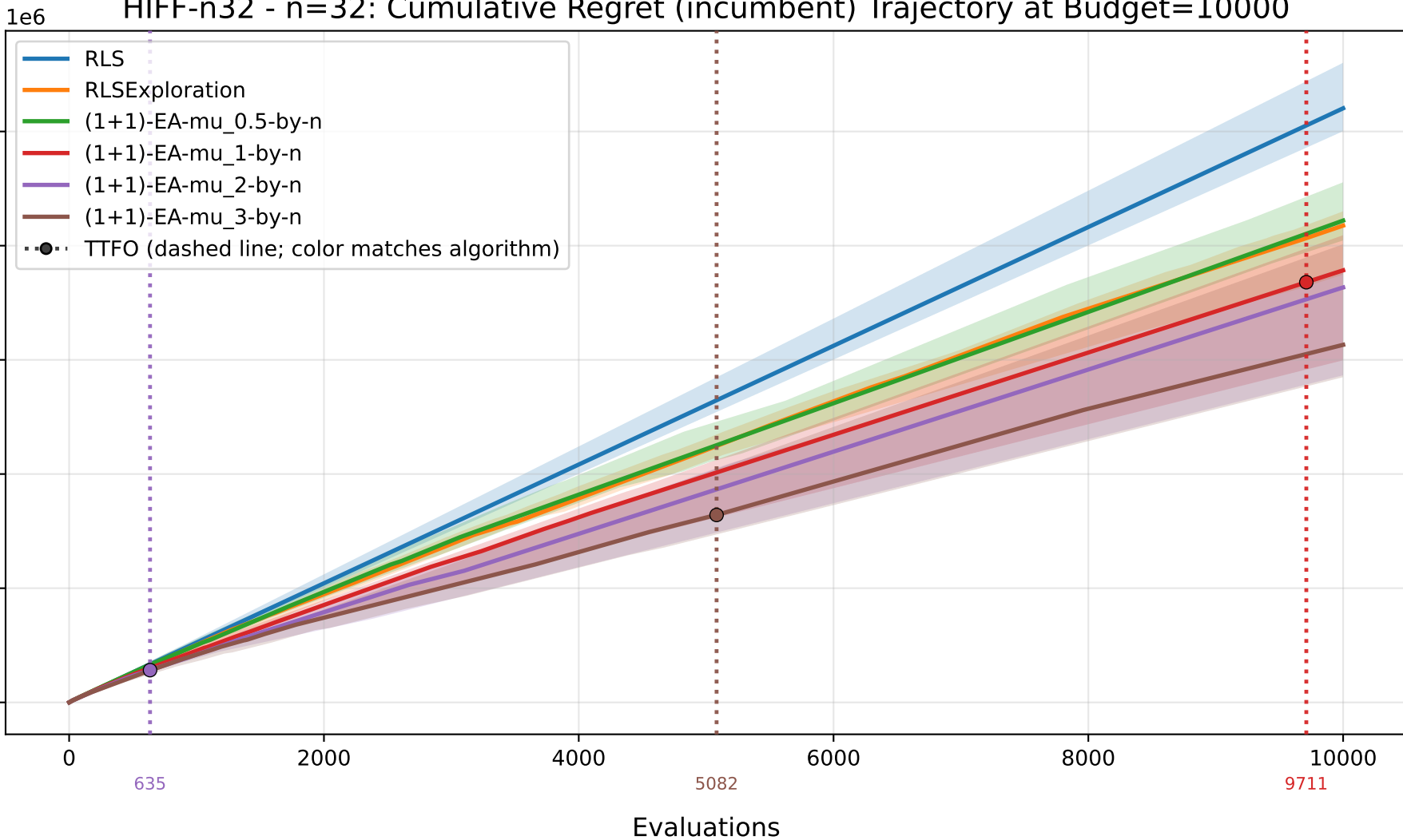
HIFF-n32 - n=32: Cumulative Regret (incumbent) Trajectory at Budget=10000
